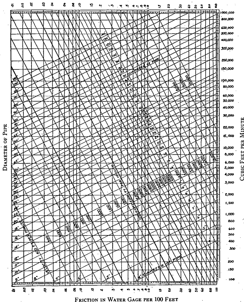
FIG. 81. FRICTION CHART
