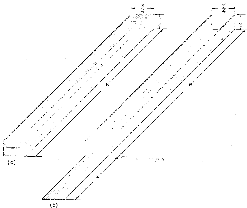
FIGURE 1. Channels used for determining rheological properties, (a) for self leveling or flow type compound (type 1), (b) for non-sag type compound (type 2)
