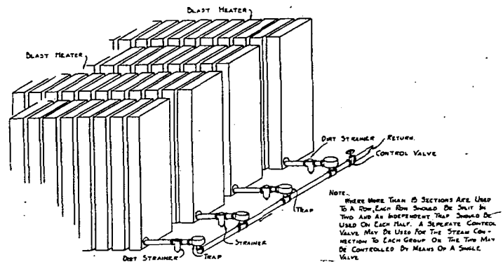
FIG. 28. RETURN CONNECTIONS TO BLAST COILS
