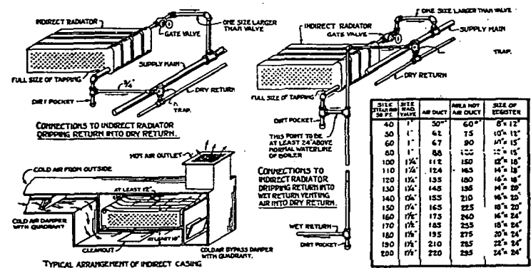
FIG. 27. INDIRECT RADIATOR CONNECTIONS
