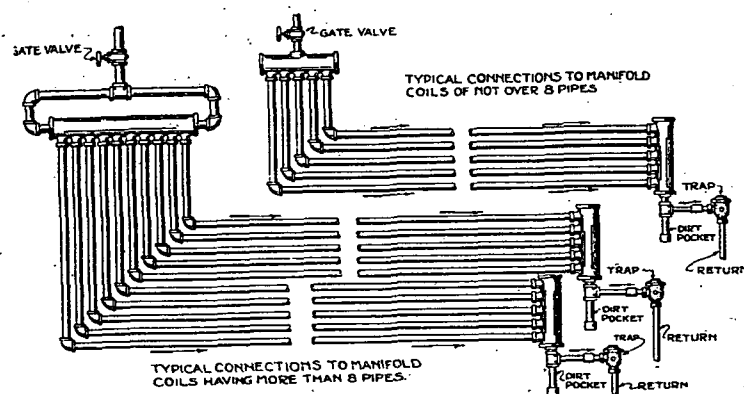
FIG. 26. TYPICAL CONNECTIONS TO MANIFOLD COILS HAVING MORE THAN 8 PIPES
