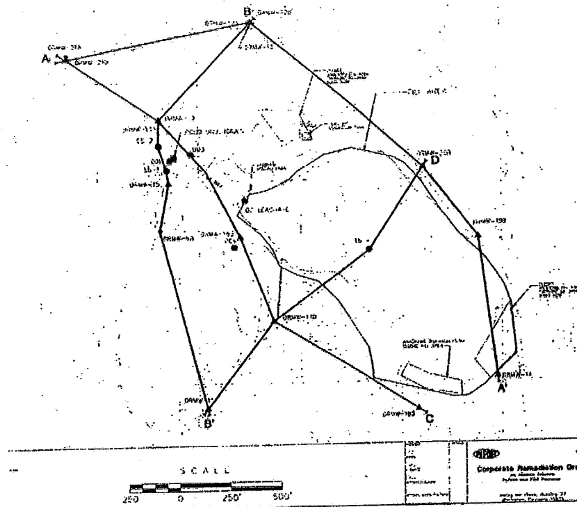
Figure 2.2: The Dry Run Landfill Geological Cross-Section Lines.
