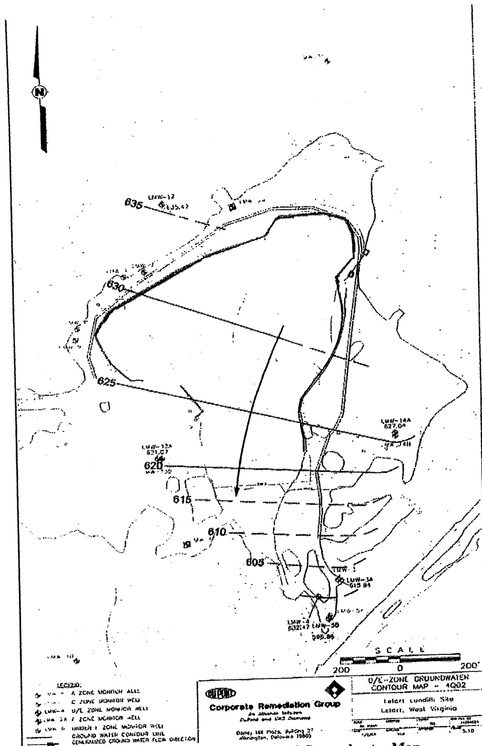
Figure 3.8: Letart Landfill Zone D-E Top-of-Groundwater Map.
