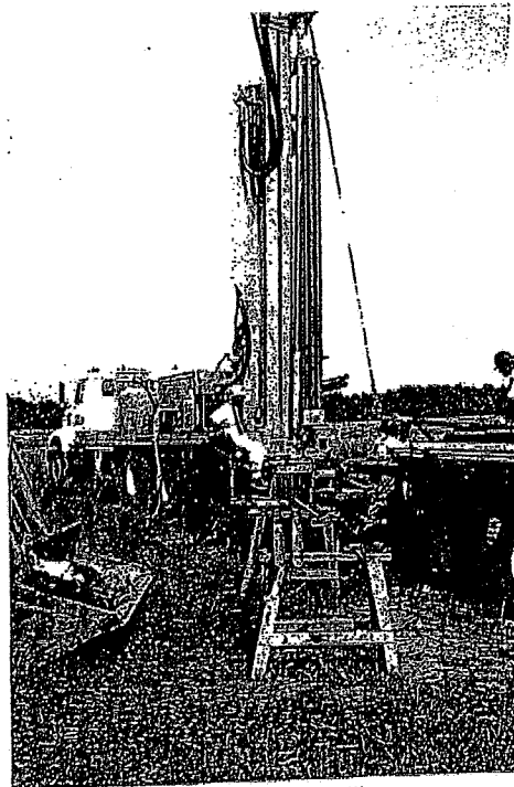
An air rotary drilling rig installing a new groundwater monitoring well at the Letart Landfill.
