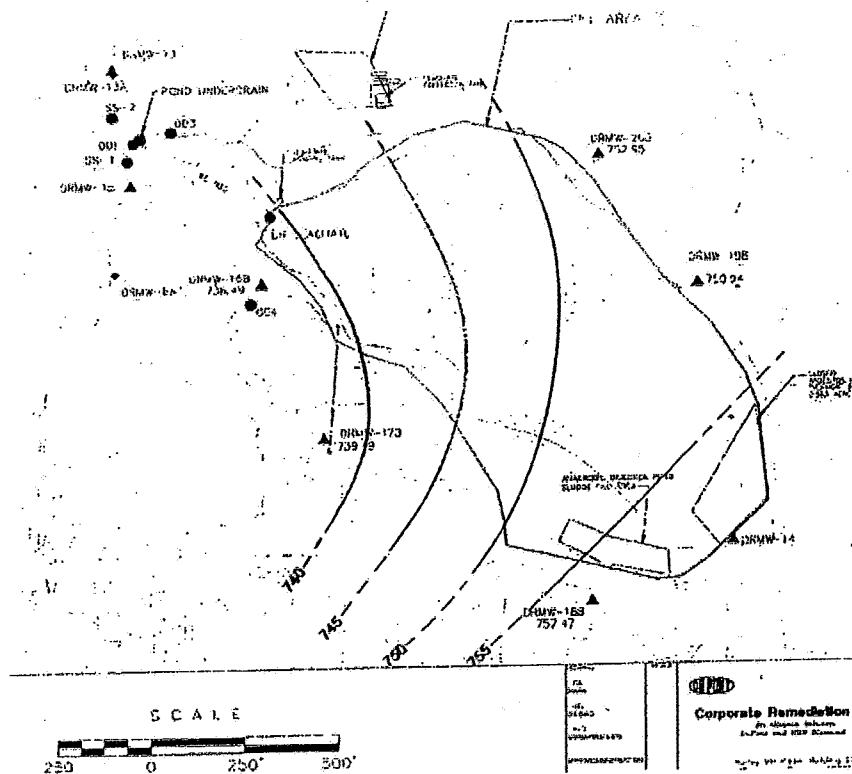
Figure 2.7: Dry Run Zone A Top-of-Groundwater Map.
