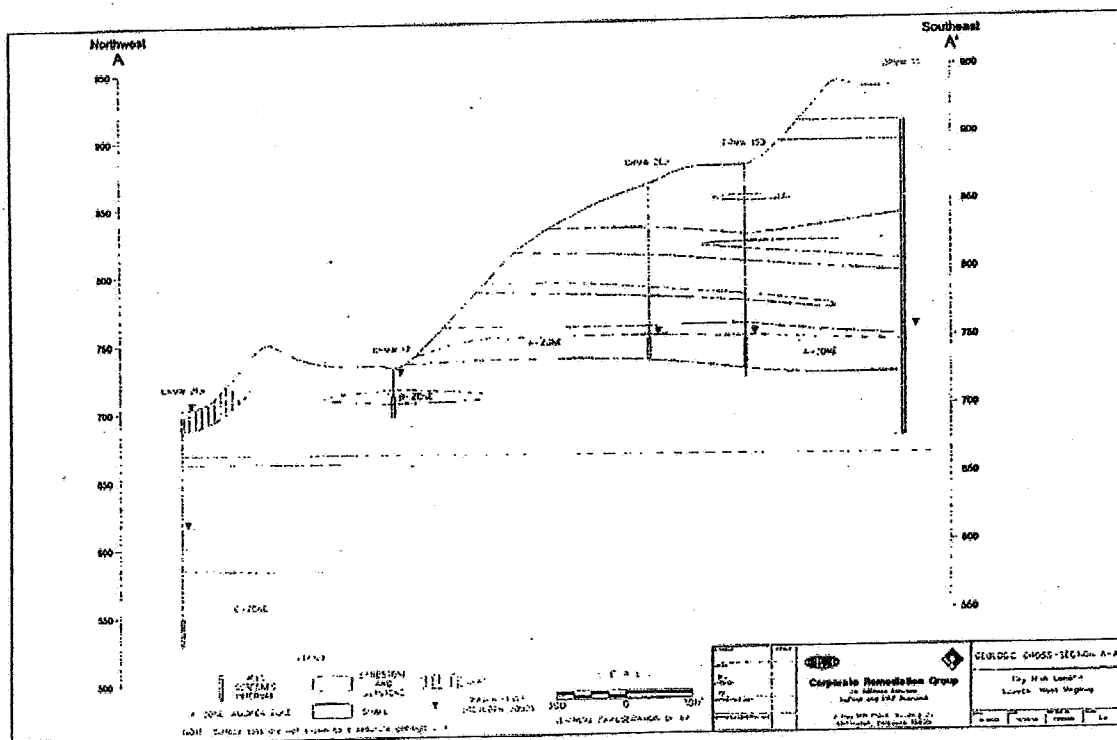
Figure 2.3: Dry Run Geological Cross-Section A-A'
