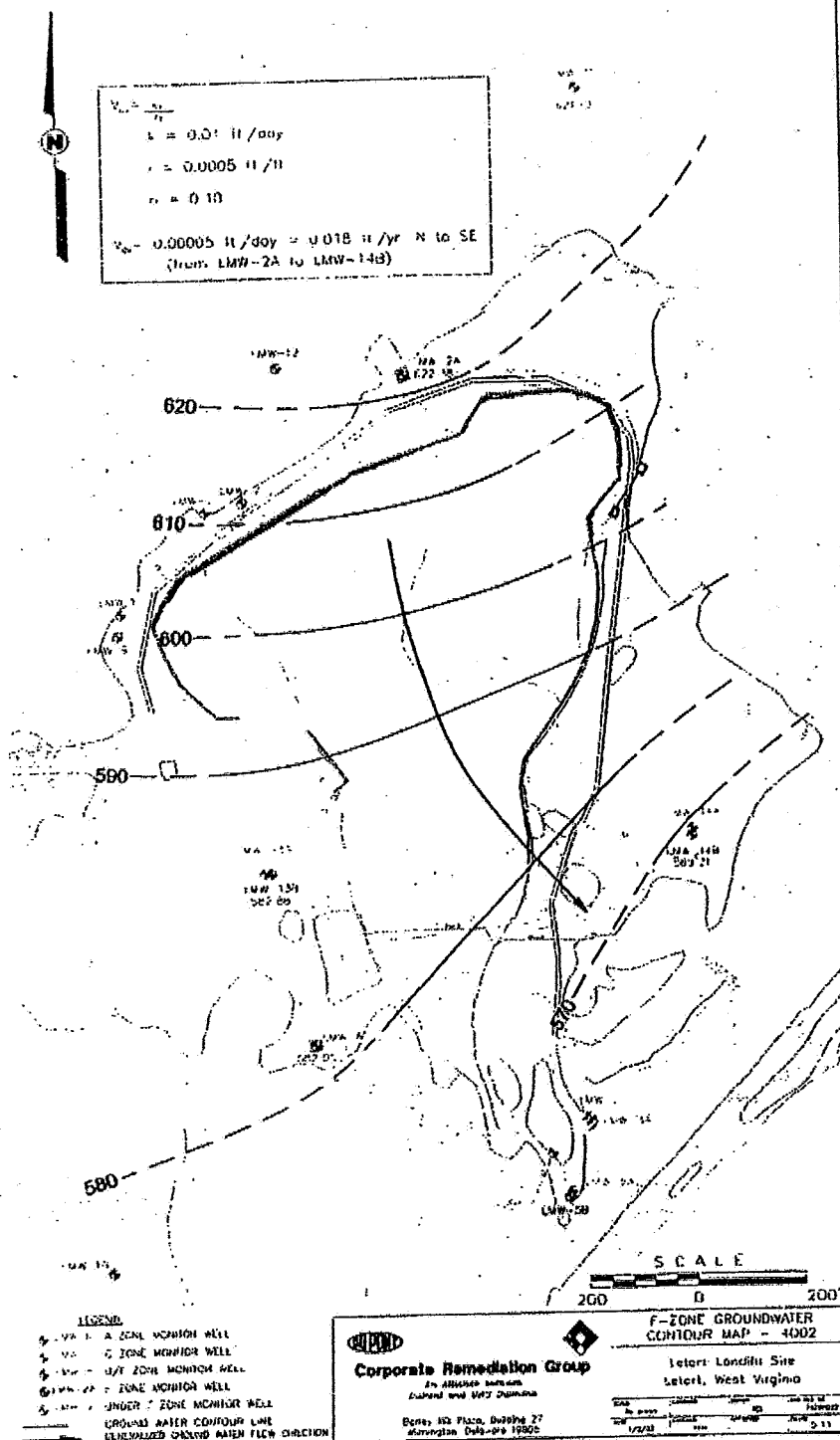
Figure 3.9: Letart Landfill Zone F Top-of-Groundwater Map.
