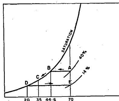
FIG. 1. TWO TYPICAL HEATING AND COOLING PROCESSES IN AIR WITHIN BUILDINGS SHOWN ON A.S.H.V.E. PSYCHROMETRIC CHART
