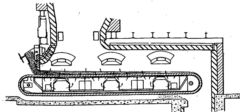
FIG. 8. OVERFEED TRAVELING-GRADE STOKER
