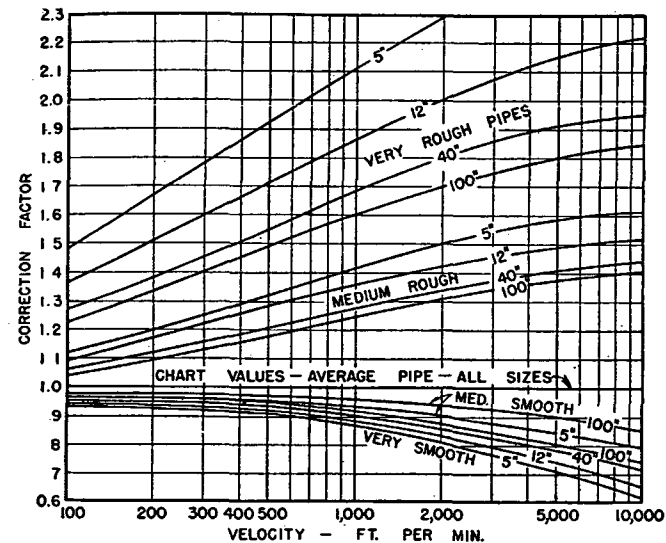
FIG. 3. CORRECTION FACTORS FOR PIPE ROUGHNESS
