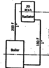
FIG. 7. GRAVITY SYSTEM
