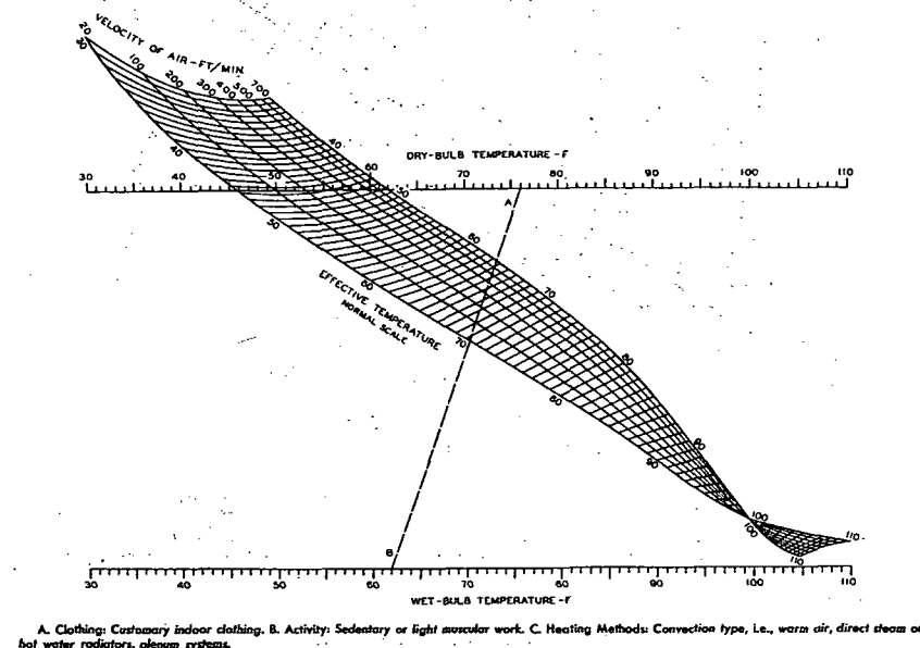
Fig. 9 . . . Effective Temperature Chart Showing Normal Scale of Effective Temperature, Applicable to Inhabitants of the United States Under Following Conditions:
