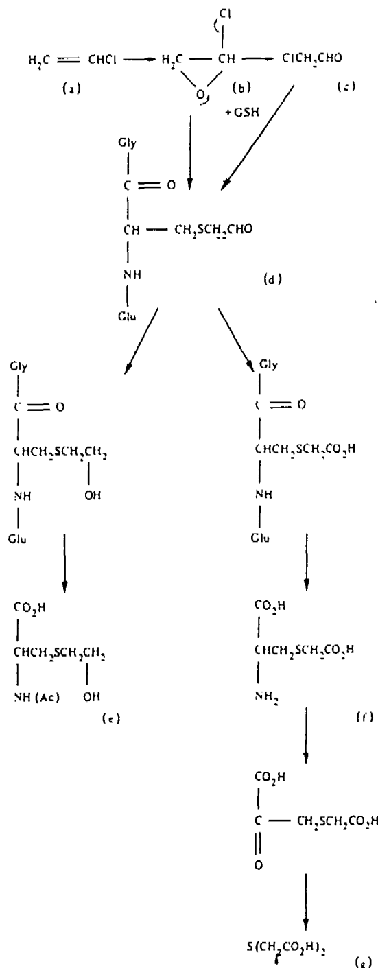
Fig. 1. Scheme showing the metabolism of vinyl chloride monomer (VCM) in rats to S-containing metabolites. VCM (a) is converted to chloroethylene oxide (b) which is transformed spontaneously to chloroacetaldehyde (c). These two metabolites are mutagenic and hence are considered to be the proximate carcinogens. The urinary excretion products N-acetyl-S-(2-hydroxyethyl)cysteine (e) S-(carboxymethyl)-cysteine (f) and thiodiglycolic acid (g) are derived from these mutagenic metabolites via (d). Gly and Glu are the glycine and glutamate residues of glutathione. [After Green & Hathway (1977)].
