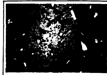
C. Actinolite
