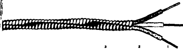
1. ENAMELED COPPER CONDUCTOR 2. POLARIZED FELTED ASBESTOS 3. COATED STEEL ARMOR
