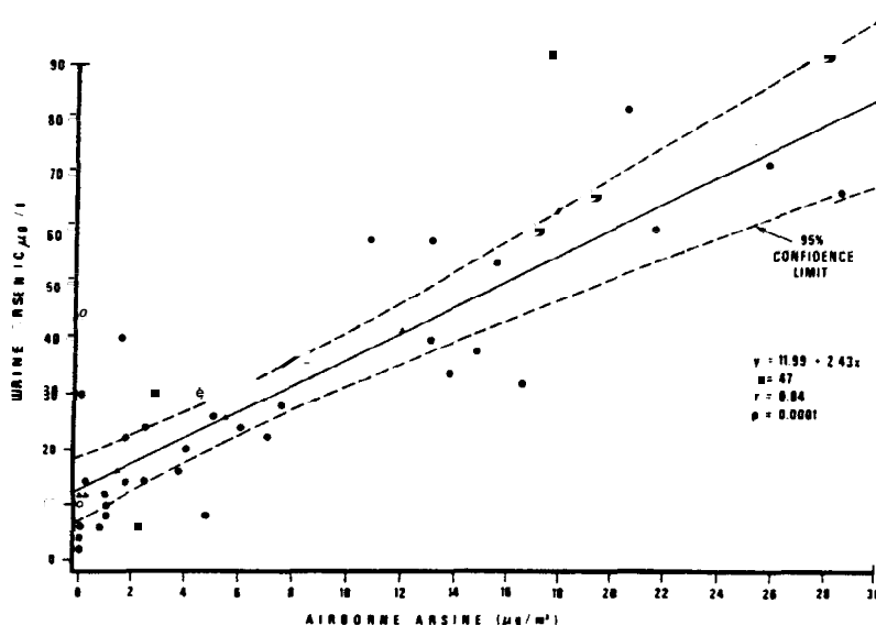
Fig 2. Correlation between arsenic exposure and urinary arsenic excretion — Lead-acid battery plant, November 1980. ( 1 \mu\text{g} arsenic/l urine = 0.01335 \mu\text{mol} arsenic/l urine)
