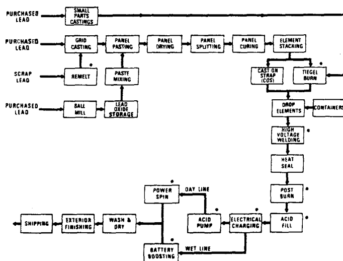
Fig 1. Process flow — Lead acid battery plant, November 1980. (* = job category with potential exposure to airborne arsenic species)
