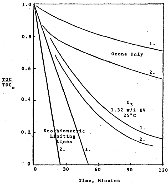
FIGURE 4. Destruction of 1. Dichlorobenzene (initial, 100 mg/l). 2. Dichlorobutane (initial, 50 mg/l).
