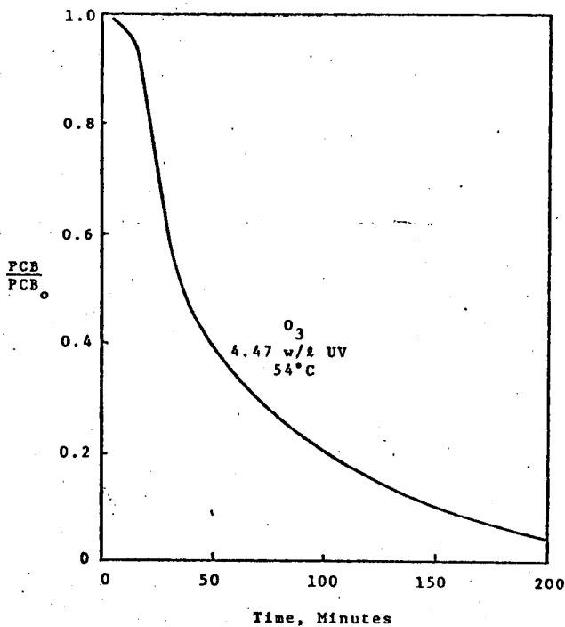
FIGURE 5. Destruction of Polychlorinated Biphenyls (PCB) (initial, 0.5 mg/l)
