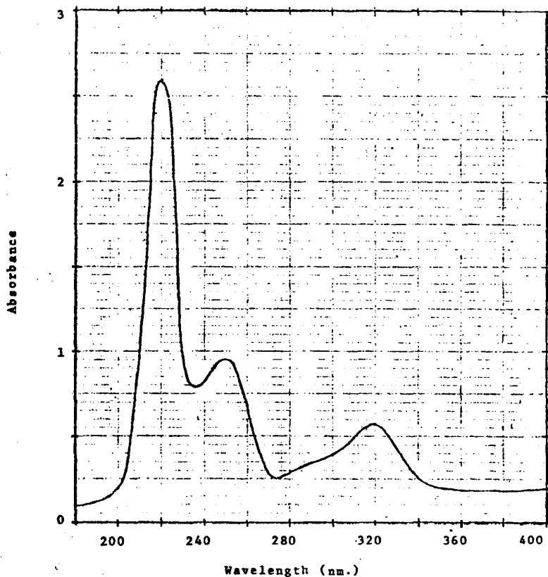
FIGURE 1. Pentachlorophenol UV-Spectrogram (7.0 mg/l)
