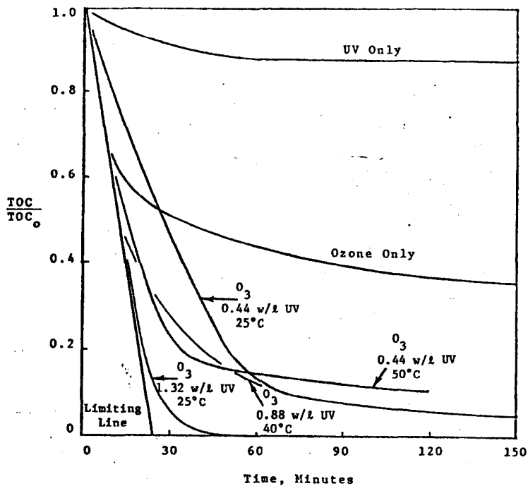
FIGURE 2. Destruction of Pentachlorophenol TOC (initial PCP, 70 mg/l)
