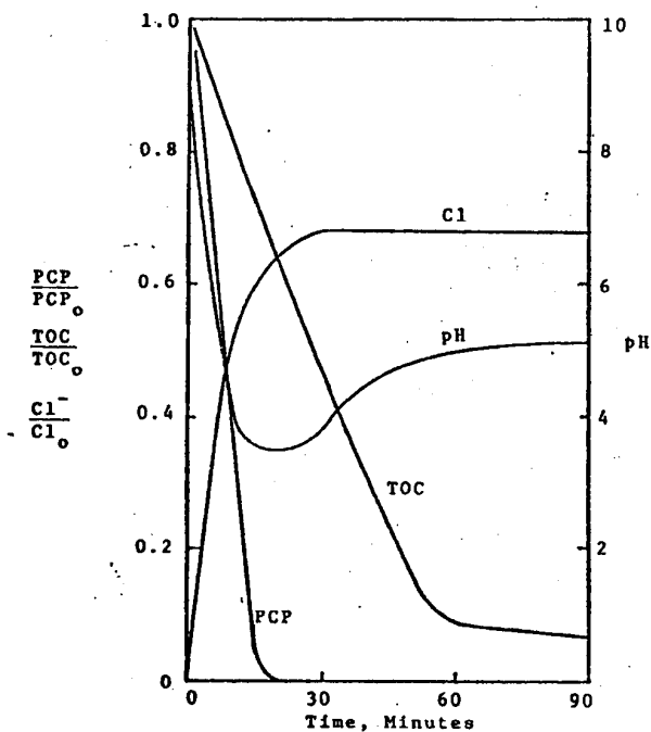
FIGURE 3. Related Time Profiles, Oxidation of Pentachlorophenol. (Re: Figure 2.)
