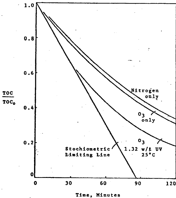
FIGURE 6. Destruction of Chloroform TOC (initial chloroform, 600 mg/l)
