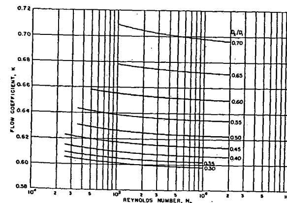
FIG. 11. FLOW COEFFICIENTS, K , FOR SQUARE-EDGED ORIFICE PLATES AND VENA CONTRACTA TAPS, IN SMOOTH PIPE NOTE: From Table 7 of Reference 2.
