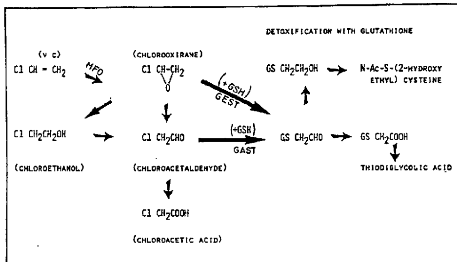
FIG. 1. The proposed metabolic fate of vinyl chloride. (GSH, glutathione; MFO, mixed-function oxidase; VC, vinyl chloride; GEST, glutathione S-epoxide transferase; and GAST, glutathione S-aldehyde transferase).
