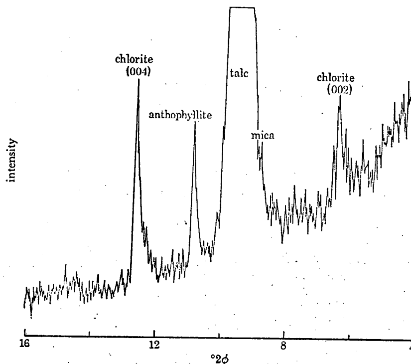
FIGURE 7. Continuous X-ray diffraction trace of consumer talcum powder purchased in New York City
