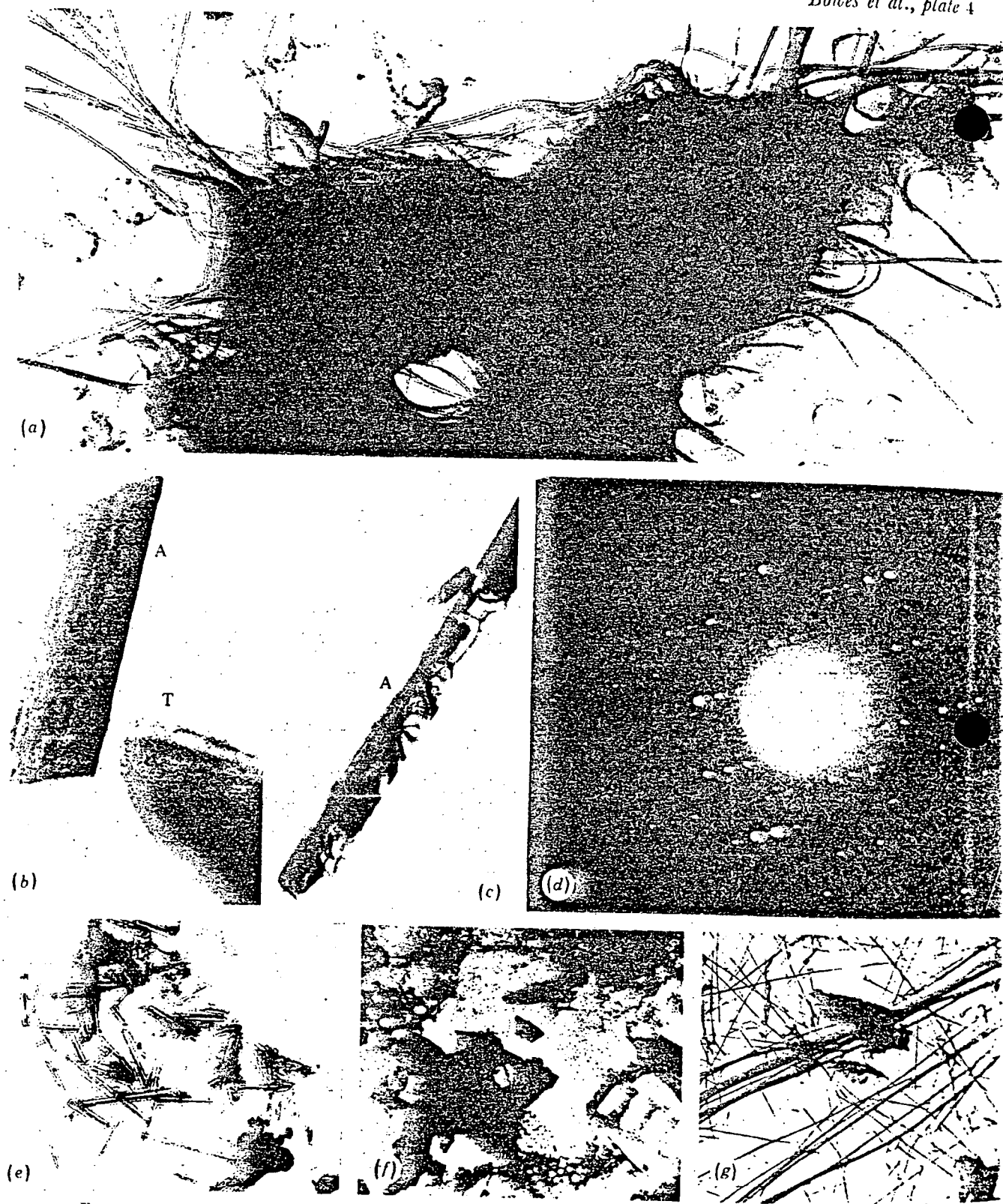
FIGURE 4. Mineral particles in water, food, drugs, tobacco sheet and clothing. (a) Chrysotile in water, Thetford, Canada; magn. \times 40000 . (b, c) Amphibole (A) and talc (T) on rice; magn. \times 20000 , \times 15000 . (d) Selected area electron diffraction pattern of amphibole in (c). (e) Asbestos in parenteral drug; magn. \times 30000 . (f) Diatom fragments and short fibres (arrowed) in low temperature ashed reconstituted tobacco sheet; magn. \times 3000 . (g) Chrysotile present (8%) in a woman's coat; magn. \times 2250 .
