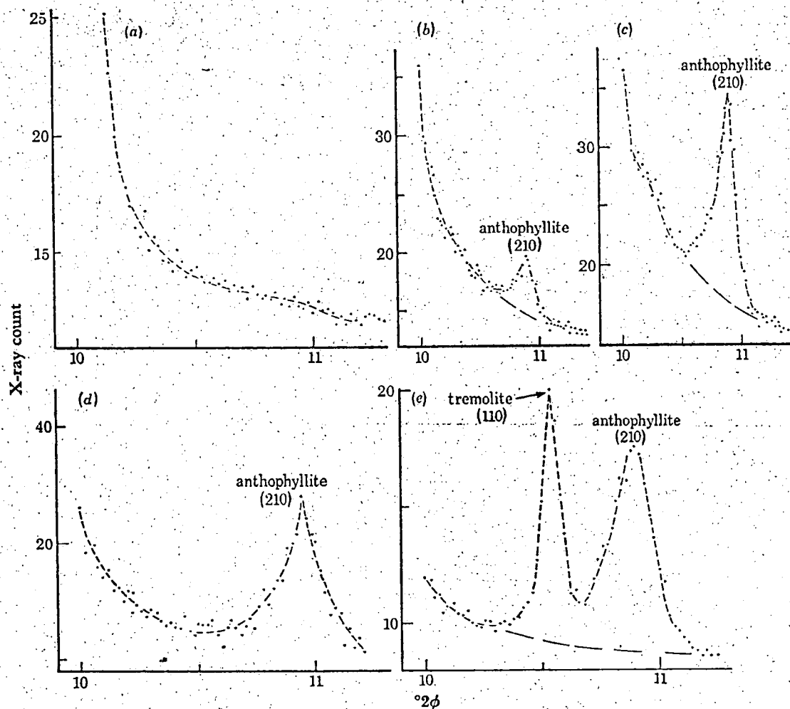
FIGURE 8. X-ray diffraction step scans of talc samples. (a, b, c) Representative dilution standards containing 1%, 5% and 10% anthophyllite in talc. (d, e) Consumer talcum powders purchased in New York City.
