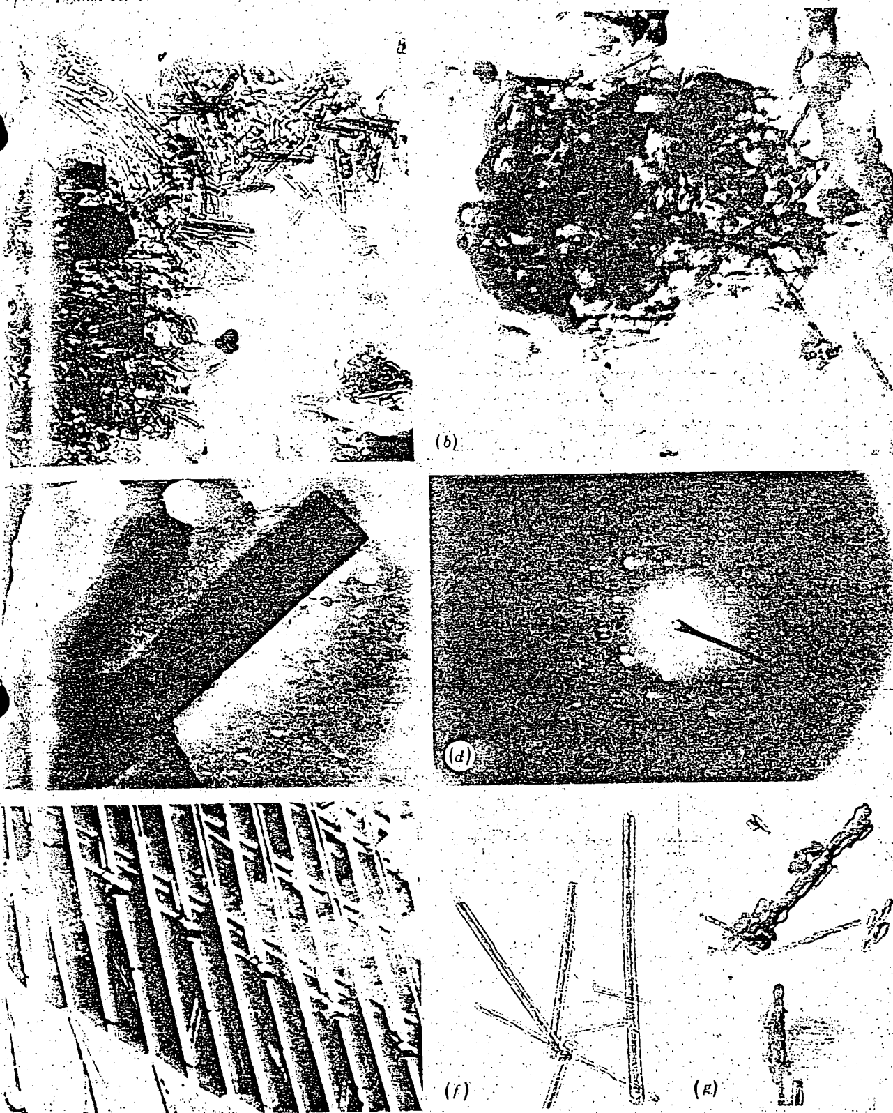
FIGURE 1. Mineral particles in the atmosphere. (a) Chrysotile in Greenland ice cap 1750; magn. \times 55000 . (b) Chrysotile in Greenland ice cap 1920; magn. \times 40000 . (c) Amphibole in Greenland ice cap 1920; magn. \times 20000 . (d) Selected area electron diffraction pattern of amphibole in (c). (e) Asbestos spray clouds at construction site, New York City. (f, g) Chrysotile in indoor air samples, New York City; magn. \times 19000 , \times 15000 .
