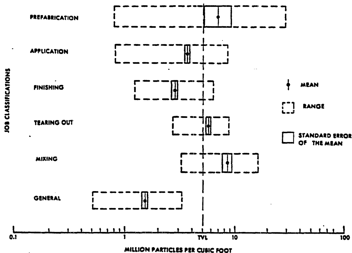
Fig. 1. Midget Impinger Counts by Job Classification.
