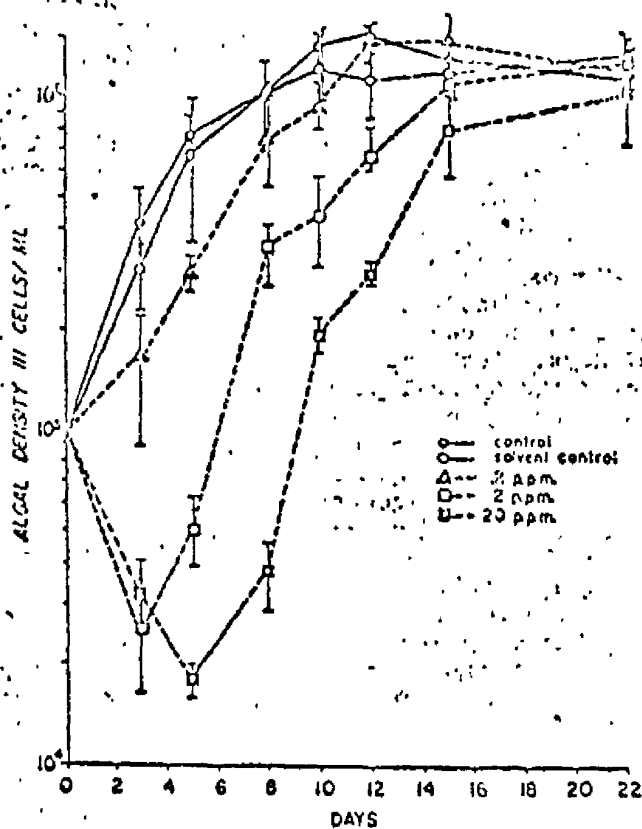
Fig. 1. Effect of the addition of 0.2, 2, and 20 ppr Aroclor 1242 on the growth of Chlamydomonas reinhardtii . Each point represents the mean of two observations whose individual values are indicated as the range.
