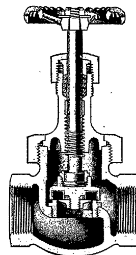
Cross Section No. 355 1/2 C, Globe All-Iron
