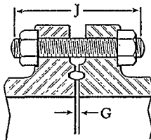
Assembled Ring Joint
