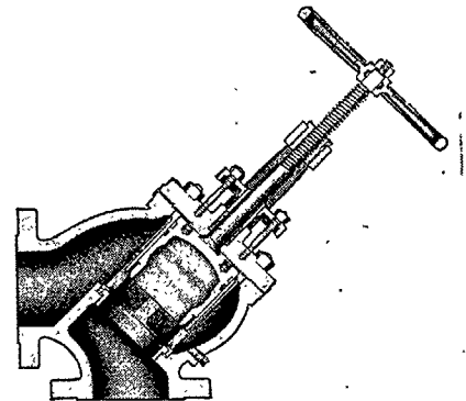
Cross Section No. 30 E, Angle Y-Pattern
