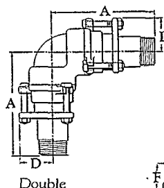
Double
