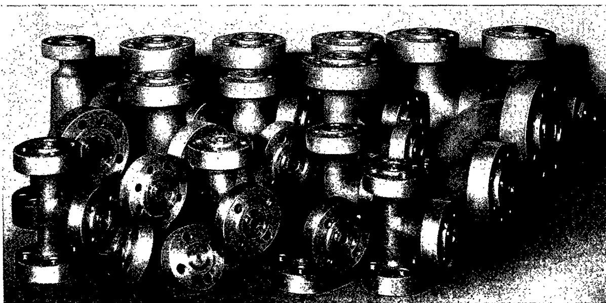
Group of Fittings for 4000-Pound Pressure Class
