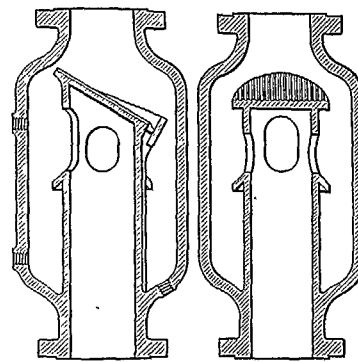
Side Section End Section Vertical Separators
