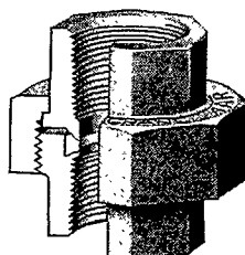
No. 950 H Union Female
