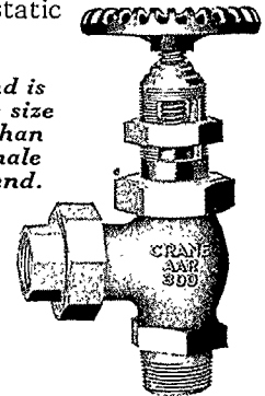
Globe, Screwed Angle, Screwed No. 1894 P, Plug Type Disc No. 1895 P, Plug Type Disc No. 1894 E, Ball Type Disc No. 1895 E, Ball Type Disc Male Inlet, Female Union Outlet
