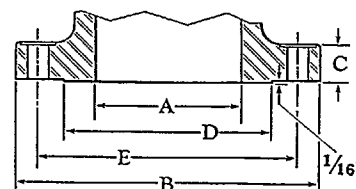
Dimensions of Flanges, in Inches
