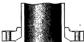
Radial Back Cranelap Joint No. 179 E, 300-Pound
