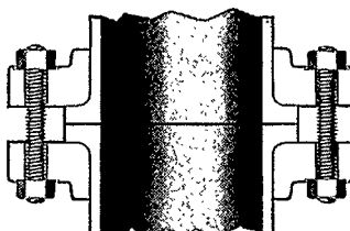
Double Thickness or 200% Lap, Cranelap Joint
