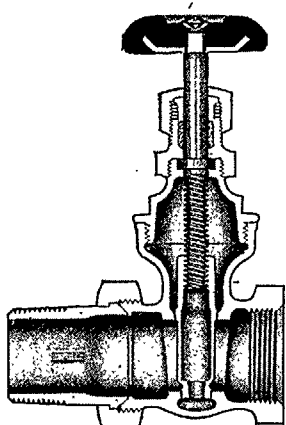
Cross Section
