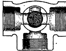
No. 268, Three-Way Square Head With Check
