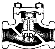
Cross Section No. 1507 1/2, Horizontal Screwed
