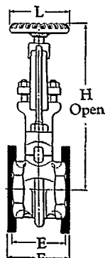
Outside Screw and Yoke
