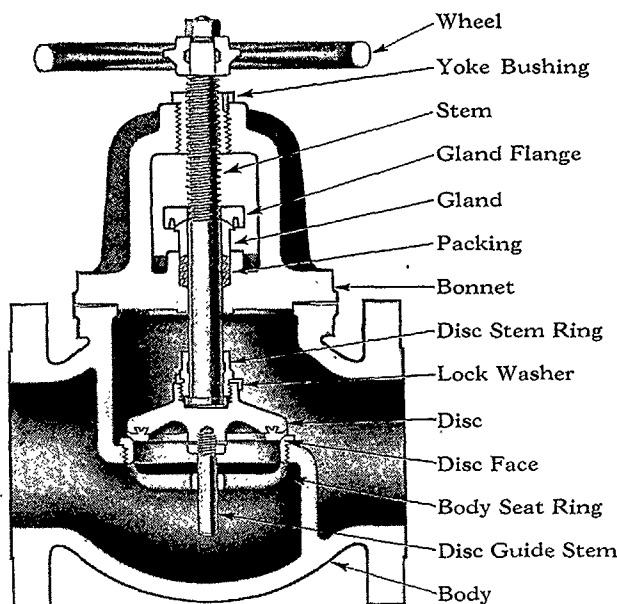
Globe Valve, Brass Trimmed
