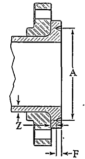
("Z" represents pipe thickness.) Cranelap Joints
