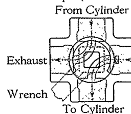
Supply Exhaust
