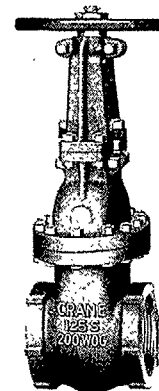
Outside Screw and Yoke Screwed No. 464 Brass Seats, Steel Stem No. 464½ Brass Seats, Brass Stem No. 475 All-Iron
