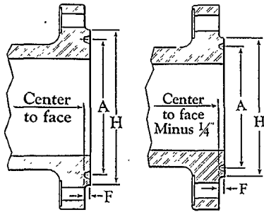
150 and 300-Pound 400, 600, 900, 1500 and 2500-Pound (See explanation of "Center to face" on next page.) For Valves, Fittings, and Flanges
