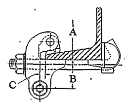
No. 226-G, Universal Channel Clamp Underwriters' Approved
