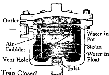
Trap Closed
