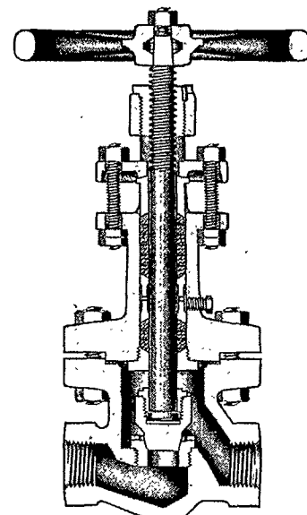
Cross Section Globe, Screwed "XR" or "U" Trimmed With Plug Type Disc and Seat
