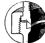
Brass to Steel Seat Used in Nos. 350 1/2 H and 350 H (Brass ring rolled in under high pressure; will not loosen in service.)
