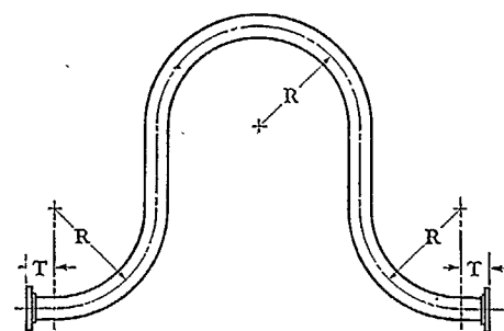
No. 9 Expansion U-Bend
