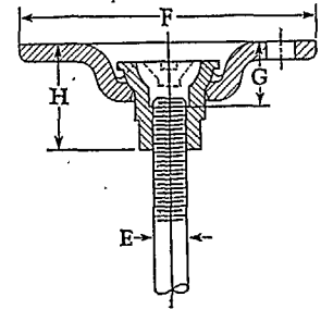
No. 154-G Swivel Hanger Flange (Cast Iron)
