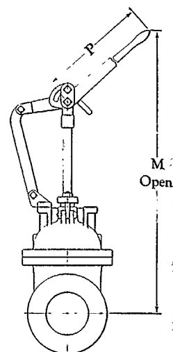
Quick Opening Valve Dimensions "E" and "F" apply also to Quick Opening Valves
