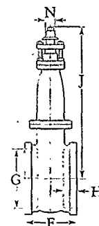
Hub Ends
