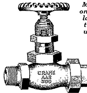
Globe, Screwed Angle, Screwed No. 1894 P, Plug Type Disc No. 1895 P, Plug Type Disc No. 1894 E, Ball Type Disc No. 1895 E, Ball Type Disc Male Inlet, Female Union Outlet
