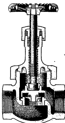
Cross Section No. 350 1/2 C, Globe Brass Trimmed
