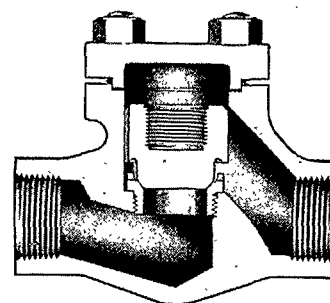
Cross Section Horizontal Check Bolted Cap
