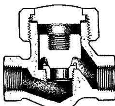
Cross Section Horizontal Check Union Cap
