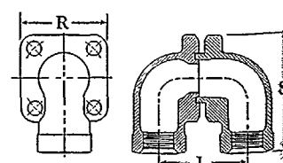
Divided Return Bend No. 1570
