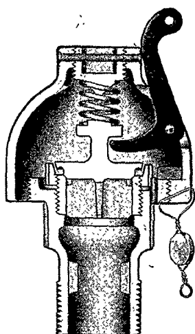
Cross Section No. 1166
