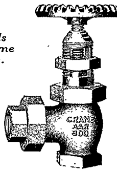
Globe, Screwed Angle, Screwed No. 1890 P, Plug Type Disc No. 1891 P, Plug Type Disc No. 1890 E, Ball Type Disc No. 1891 E, Ball Type Disc Female Inlet, Female Union Outlet
