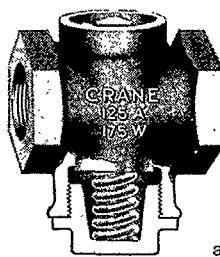
No. 318 Triangular Head With Lock Shield With Brass Plug
