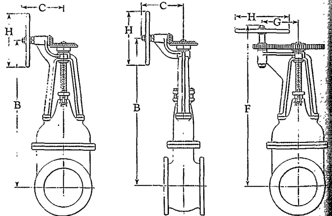
Outside Screw and Yoke Valves with Bevel or Spur Gears
