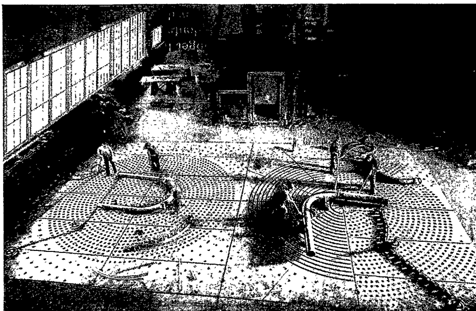
A "close-up" of 300-Pound Main and Auxiliary Steam Headers with an 8-inch Expansion Bend in the Main Header.
