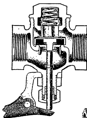
Cross Section No. 12 1/2
