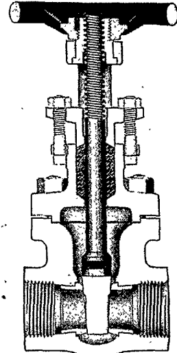
Cross Section No. 3607 W, Screwed Bolted Bonnet
