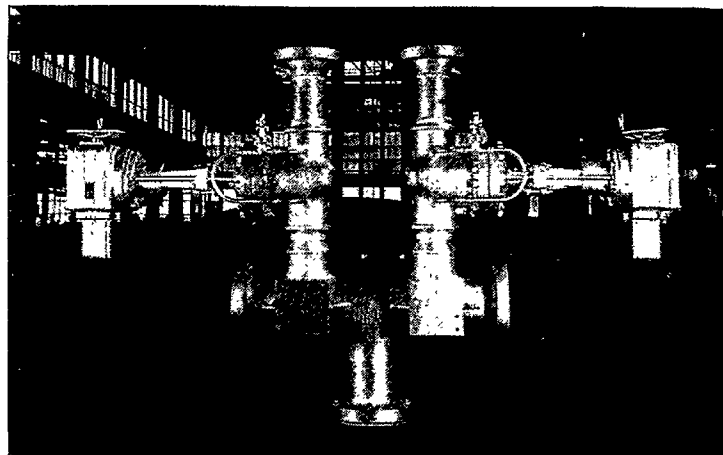
A 900-Pound Header, complete with Valves
