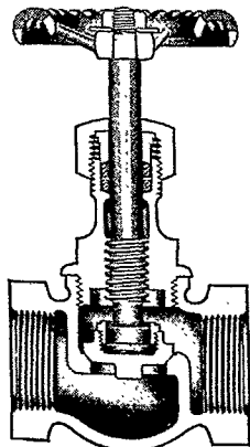
Cross Section No. 4, Globe
