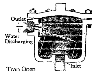
Trap Open
