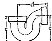
No. 1059 1 / 2 Bath P Trap
