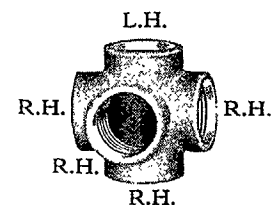
Side Outlet Cross No. 66, Right Hand No. 66½, Tapped as shown
