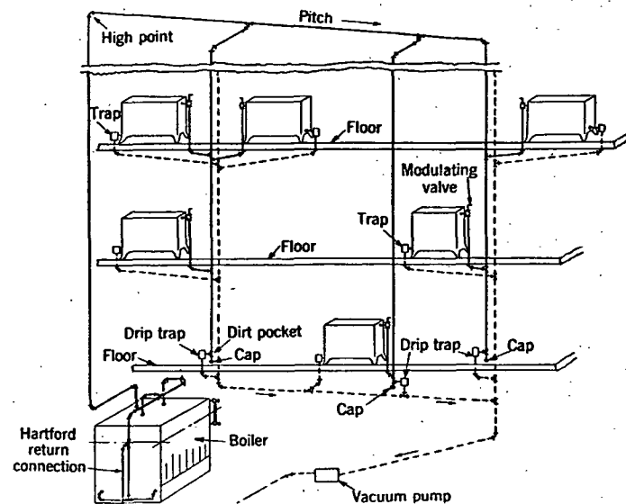
FIG. 15. TYPICAL DOWN-FEED VACUUM PUMP SYSTEM
