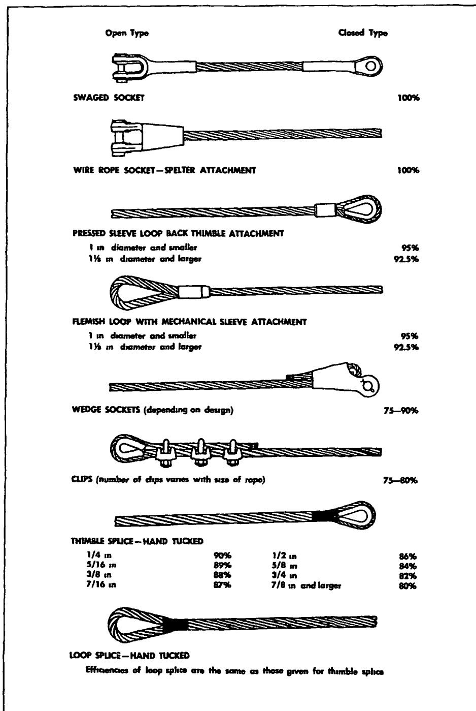
FIG 23-4 — Efficiencies of attaching wire rope to fittings in percentages of strength of rope
