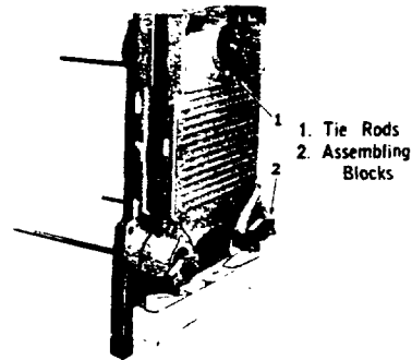
FIG. 2—Assembling Sections
