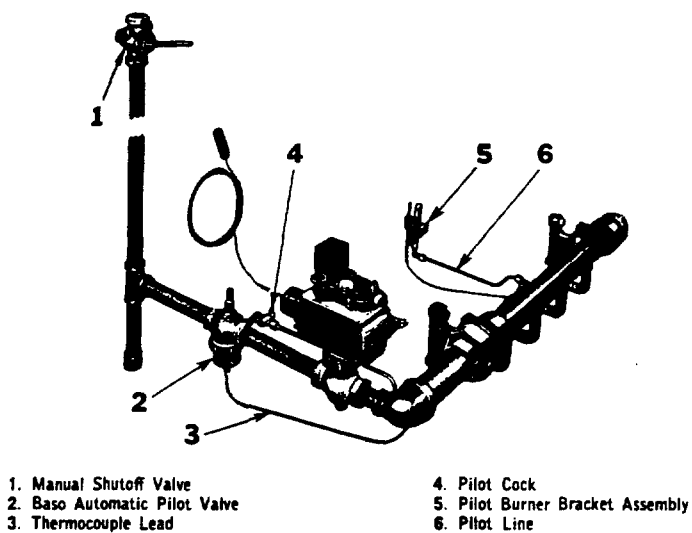
FIG. 18—Control Connections
