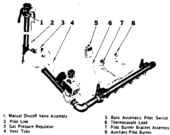
FIG. 16—Control Connections
