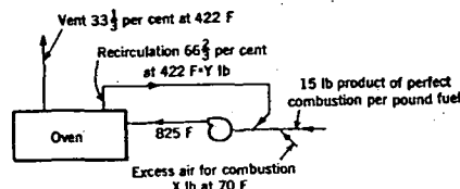
FIG. 11. CORE DRYING DIAGRAM OF COMBUSTION PRODUCTS AND AIR
