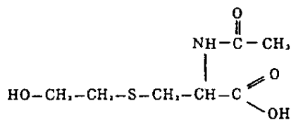
Metabolite A: N -Acetyl( S -2-hydroxyethyl)cysteine
