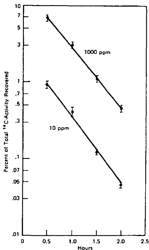
FIGURE 6. Expired vinyl chloride expressed as percentage of the recovered radioactivity vs. time following a 6-hr exposure to 10 and 1000 ppm VC. Each point represents the mean \pm standard error of the mean of four rats. The curves were fit by linear regression analysis.
