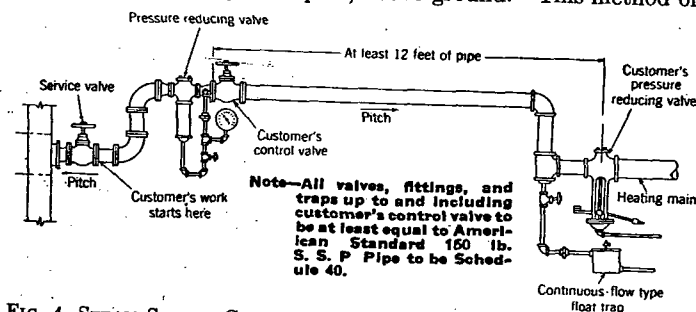
FIG. 4. STEAM SUPPLY CONNECTION WHEN USING TWO REDUCING VALVES
