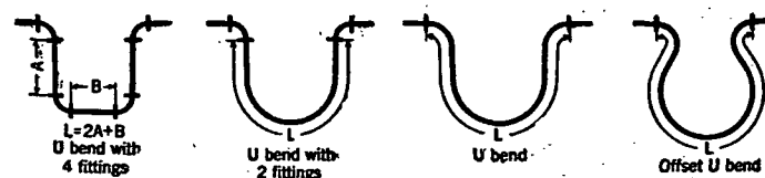
FIG. 3. MEASUREMENT OF L ON VARIOUS PIPE BENDS
