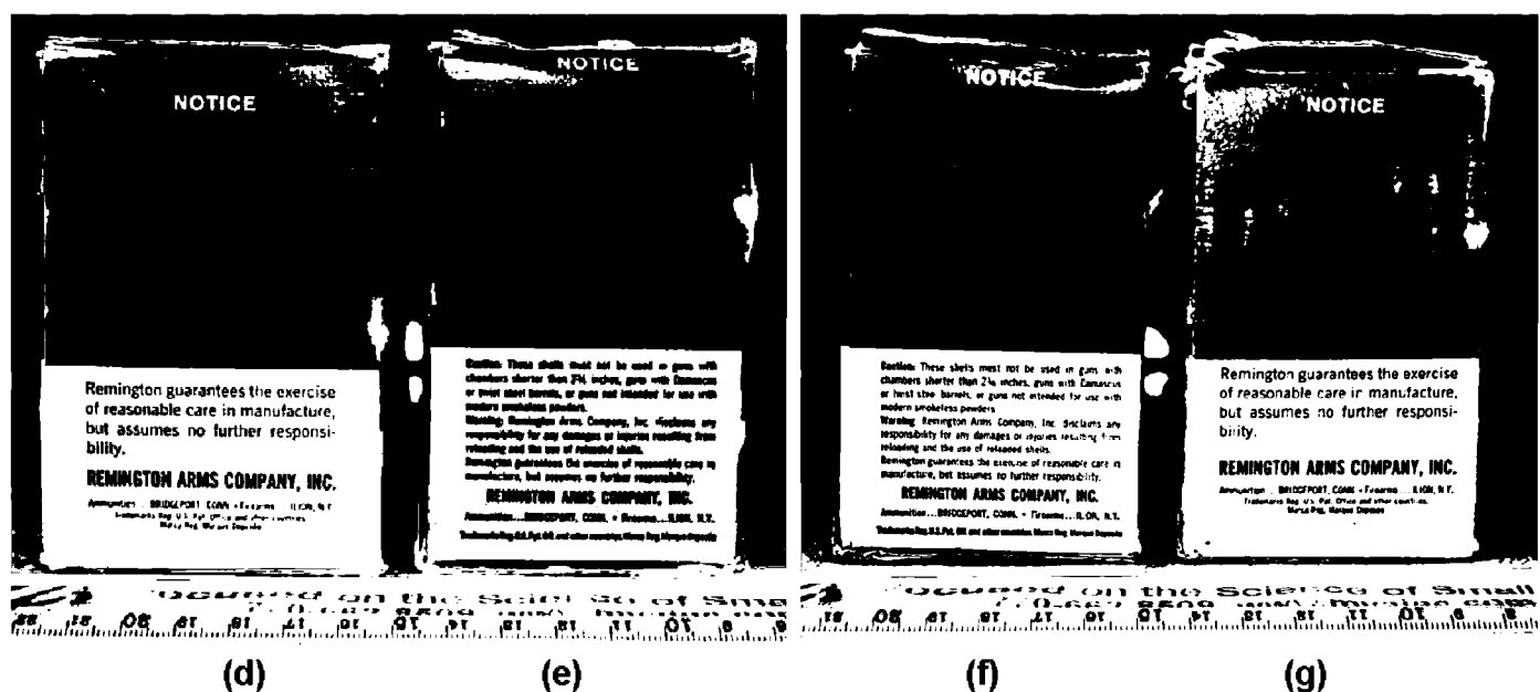
Figure 6. Remington 12 gauge shotgun shells in boxes, as received, samples (a) AE1386, (b) AE1387, (c) AE1388, (d) AE1389, (e) AE1390, (f) AE1391, (g) AE1392.
