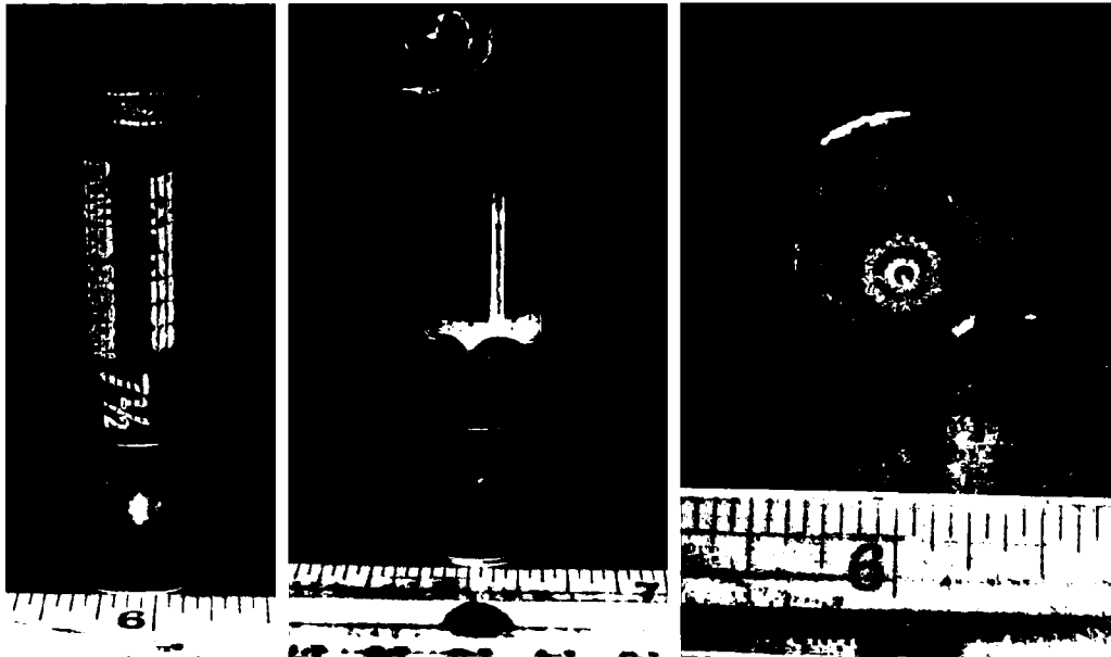
Figure 25. Dissection of sample AE1391 from left to right showing: uncut, shot removed to show shot holder, and basewad.
