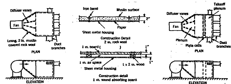
FIG. 7. ABSORPTION PLENUMS WITH AND WITHOUT SOUND CELLS
