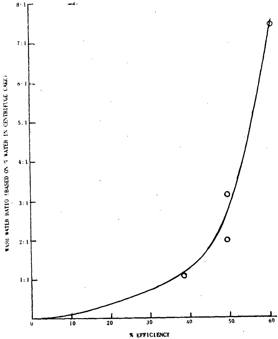
FIGURE 12. WASH WATER EFFICIENCY
