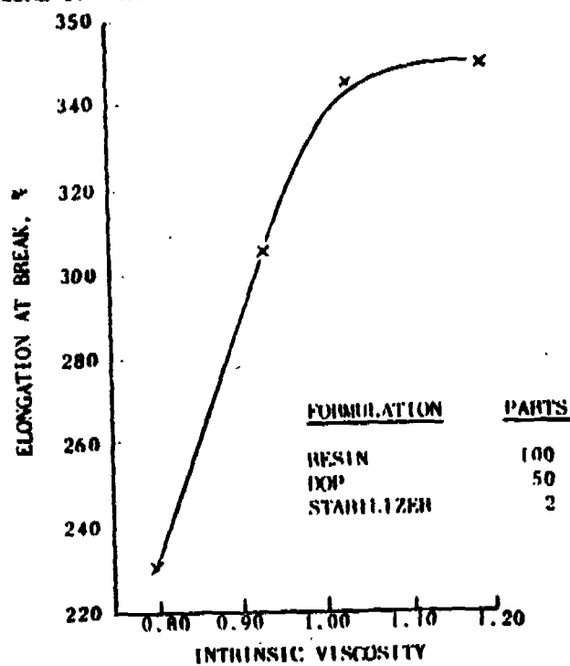
FIGURE 3. EFFECT OF MOLECULAR WEIGHT ON ELONGATION
