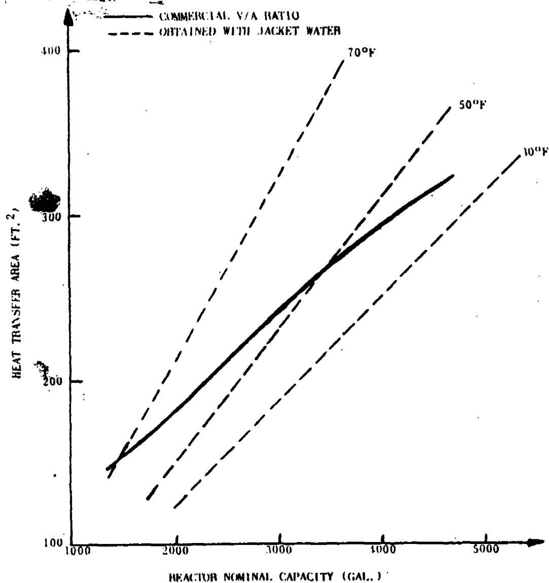
FIGURE 5. REACTOR NOMINAL CAPACITY VS. HEAT TRANSFER AREA
