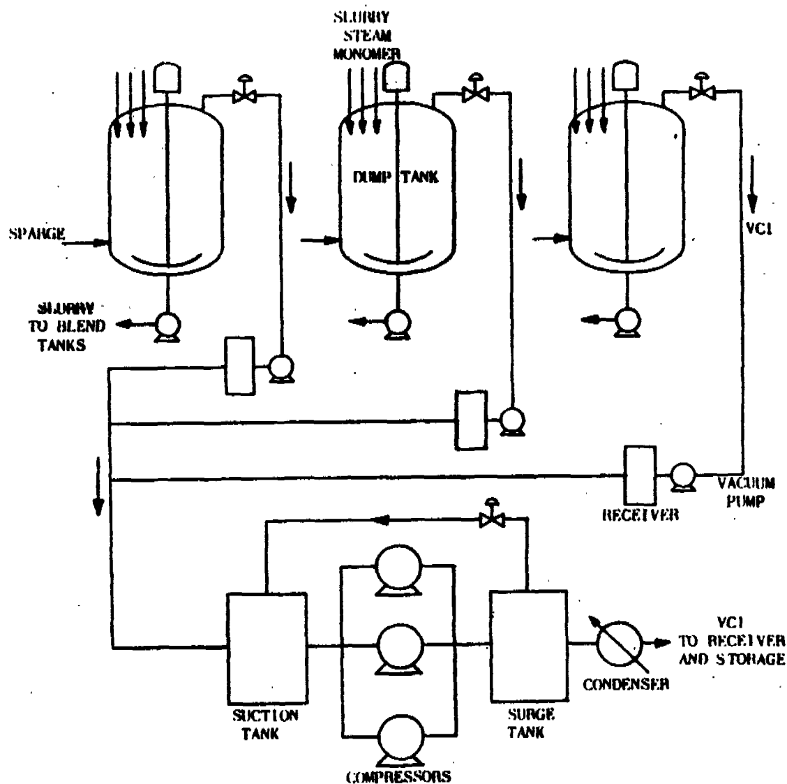
FIGURE 10. ASHTABULA RECOVERY SYSTEM
