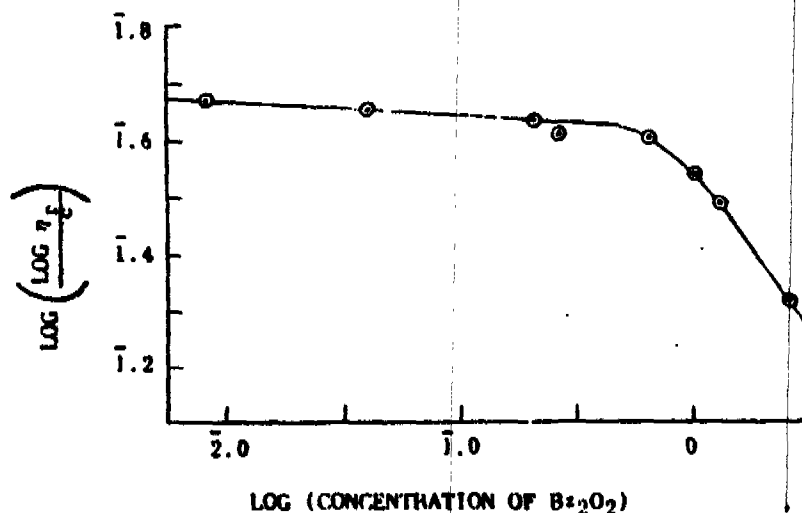
FIGURE 7. EFFECT OF CHANGE IN CATALYST CONCENTRATION ON THE AVERAGE MOLECULAR WEIGHT
