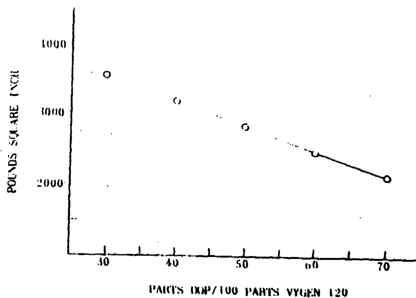
FIGURE 5. EFFECT OF DOP LEVEL ON TENSILE STRENGTH
