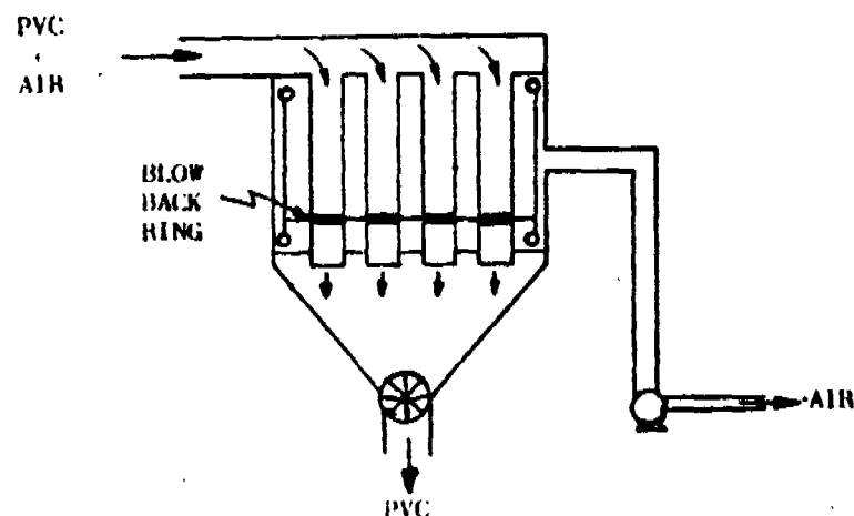
FIGURE 14. BAG FILTER
