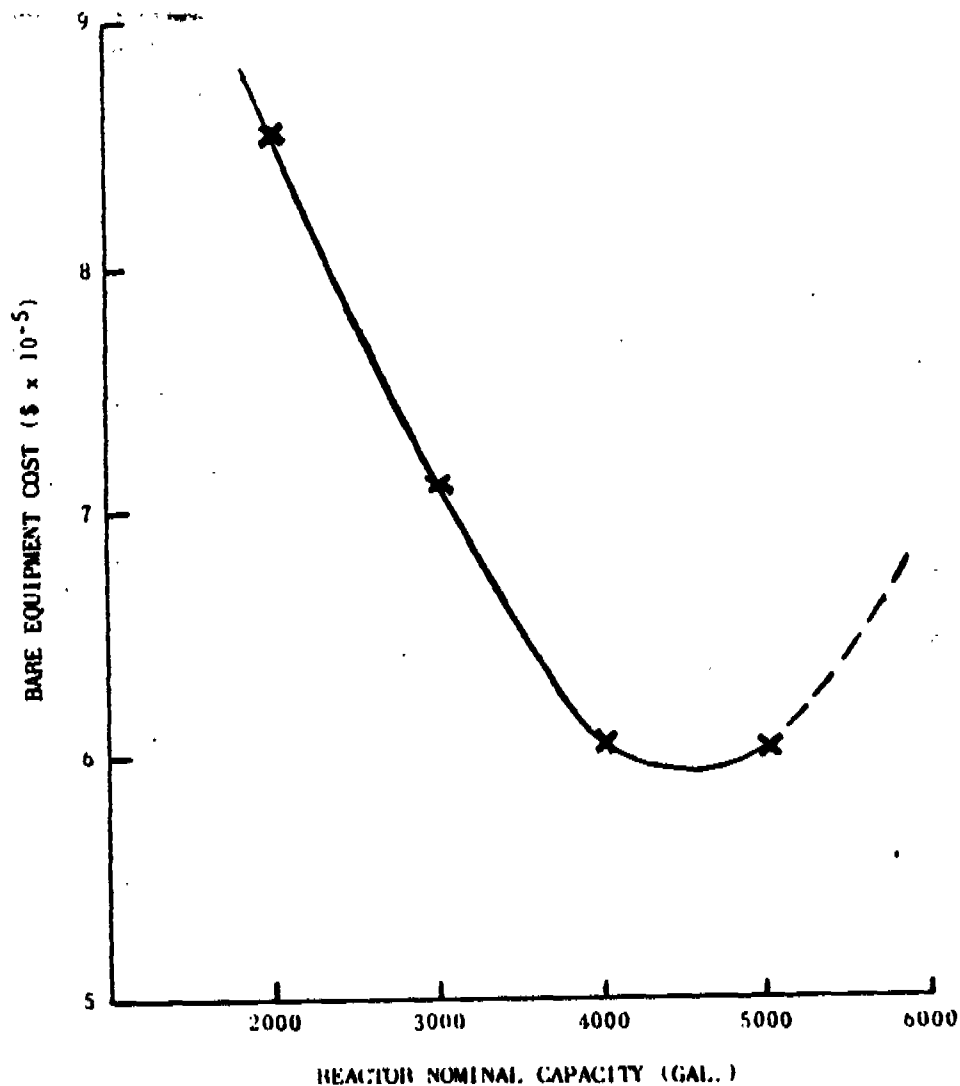
FIGURE 6. BARE COSTS VS. REACTOR SIZE
