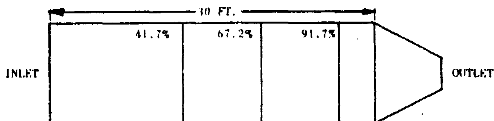
FIGURE 13. DRIER SAMPLE POINT AND BAFFLE LOCATION
