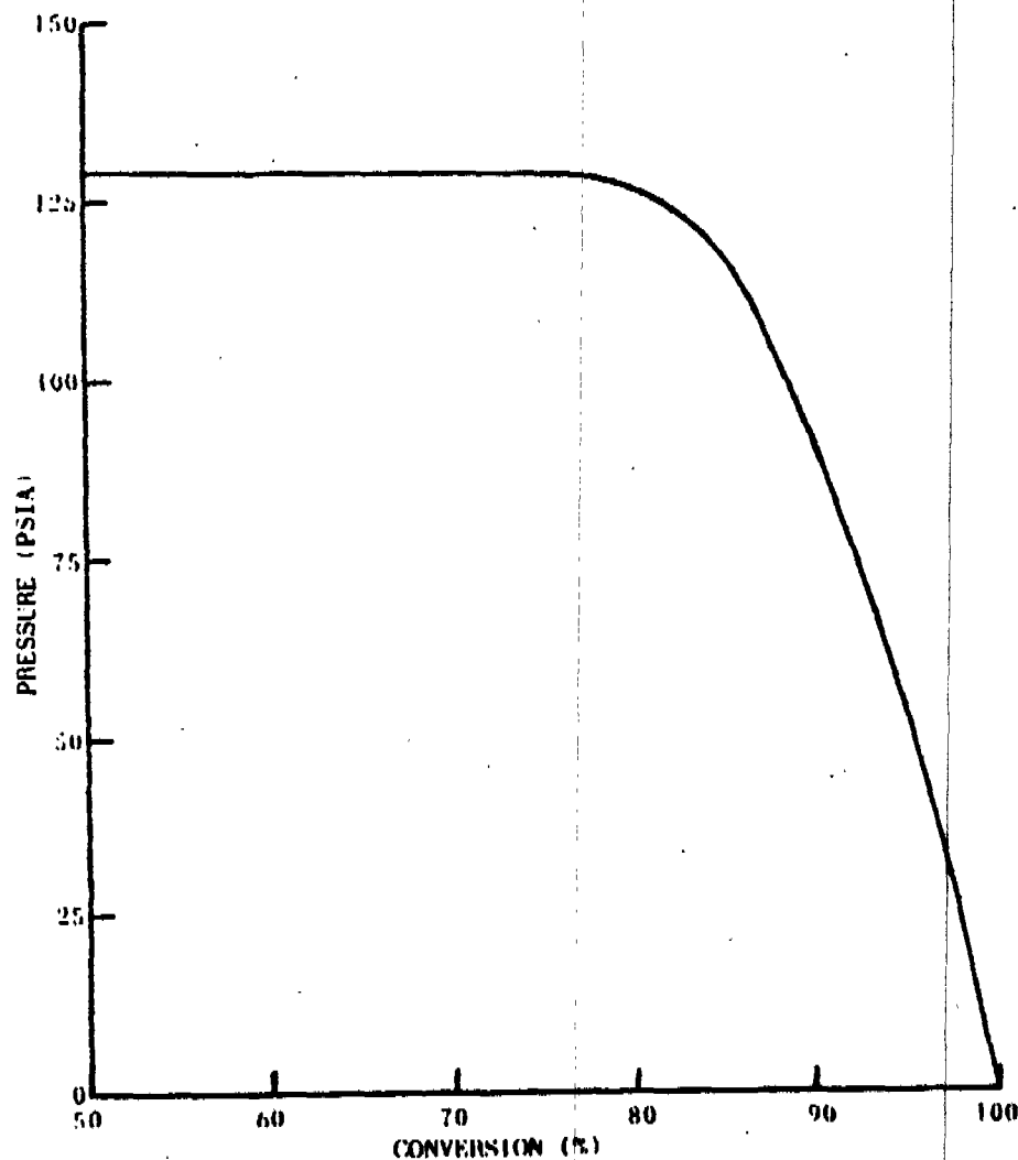
FIGURE 2. PRESSURE VS. % CONVERSION
