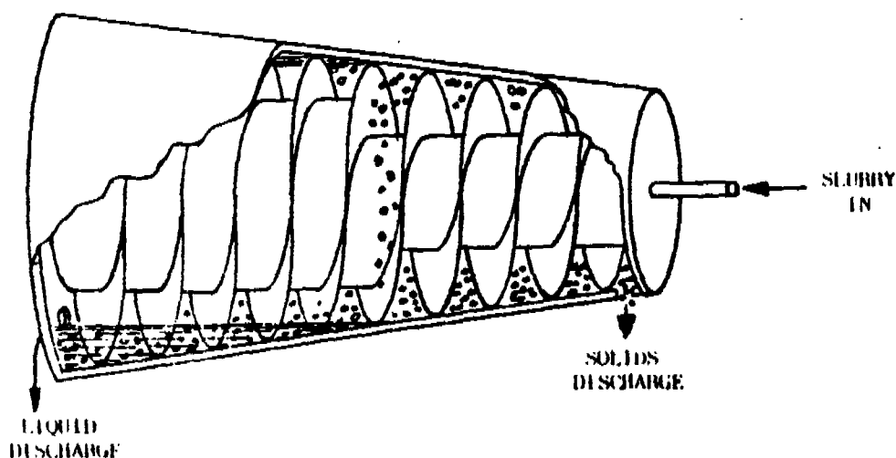
FIGURE 11. COMMERCIAL CENTRIFUGE
