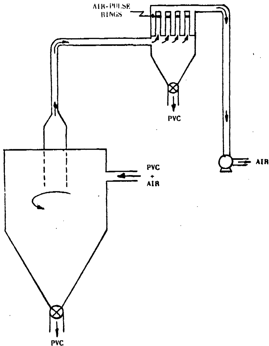
FIGURE 16. COMBINATION FILTER
