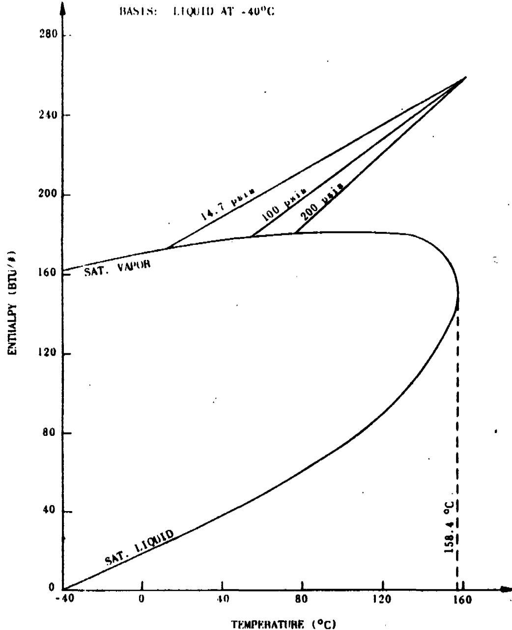
FIGURE 9. ENTHALPY OF VCI
