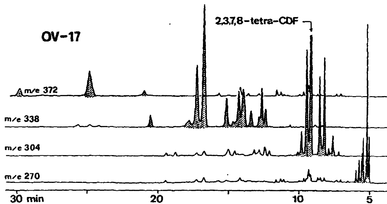
Figure 2 : Mass fragmentograms (OV-17 plus capillary column at 207°C) of Yusho oil showing elution of PCDFs ( m/e 270 = tri-, m/e 304 = tetra-, m/e 338 = penta- and m/e 372 = hexa-CDF).
