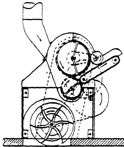
FIG. 11.—CARD WASTE END MACHINE.
