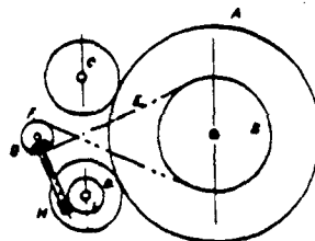
Dimensions: A-Cylinder 60" B-Brush 24" C-Driver 24" D-E-F-G-H-12"
