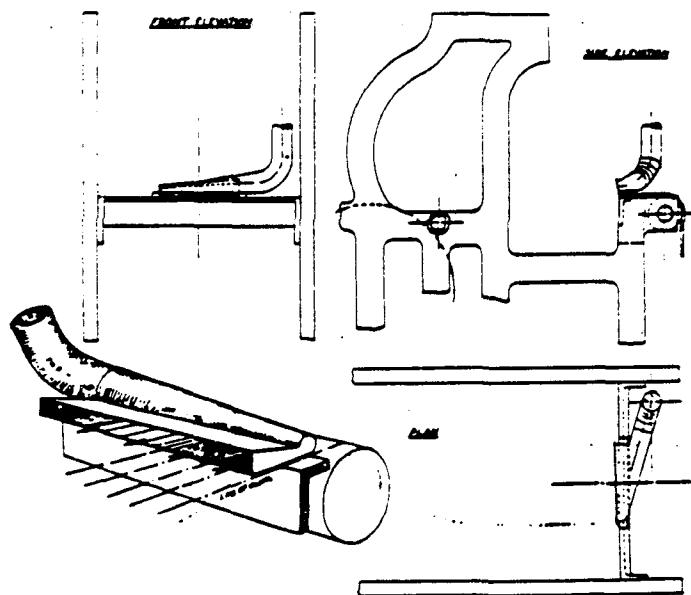
FIG. 15.—EXHAUST VENTILATION AT BRAKE BAND LOOMING LOOM. Applied at Breast.
