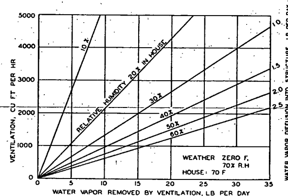
FIG. 10. WATER VAPOR BALANCE IN A DWELLING (Vapor Barrier, 1 perm; Wall and Ceiling Area 2000 sq ft Insulated)
