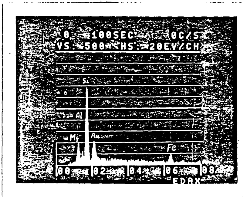
Photo 6A - Spot Mode of Particle Shown Above
