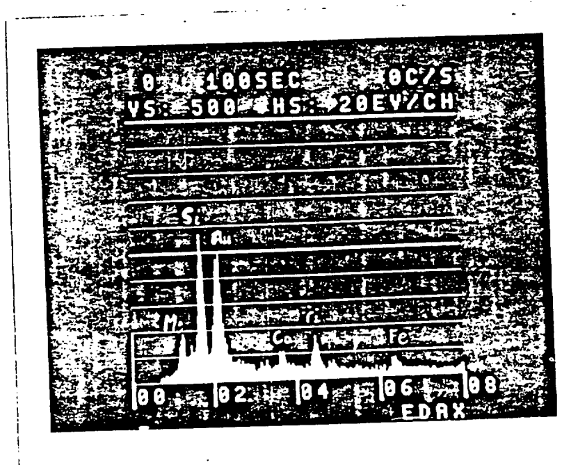
Photo 5A - Spot Mode of Fiber in Above Photo
