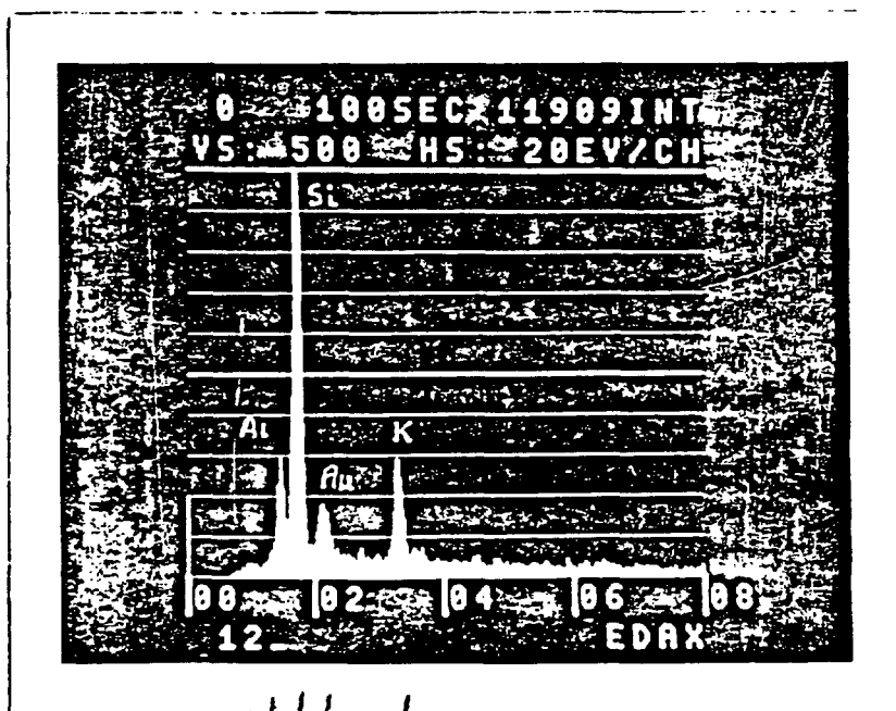
Photo 3A - Spot Mode of Particle Shown Above
