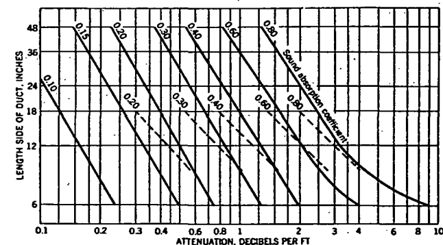
FIG. 5. SOUND ATTENUATION FOR VARIOUS ABSORBING DUCT LINERS
