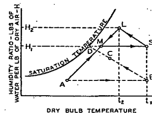
FIG. 9. CHANGES IN AIR DURING DRYING PROCESS
