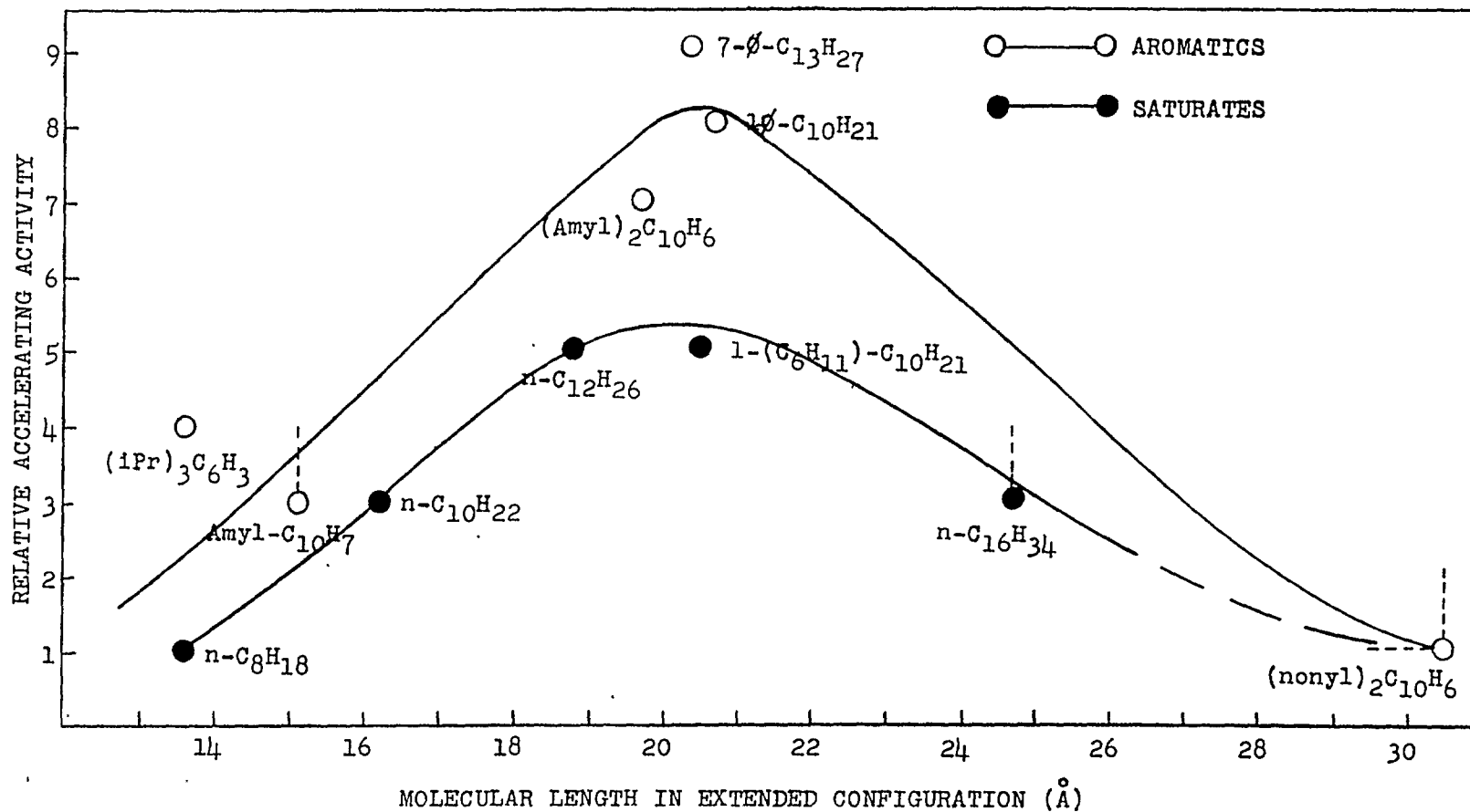
FIGURE 2 - MOLECULAR LENGTH OF SOLVENT vs. ACCELERATING ACTIVITY
