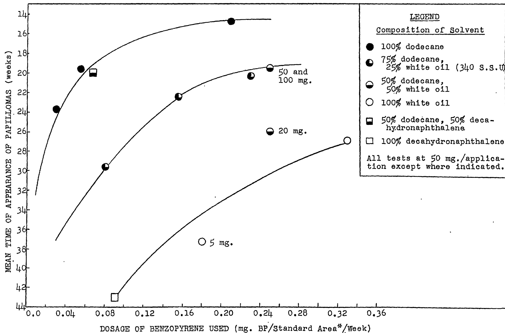
FIGURE 1 - INFLUENCE OF CYCLOPARAFFINIC DILUENTS ON THE ACCELERATING ACTIVITY OF n-DODECANE
