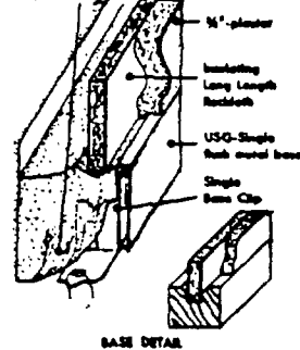
BASE DETAIL
