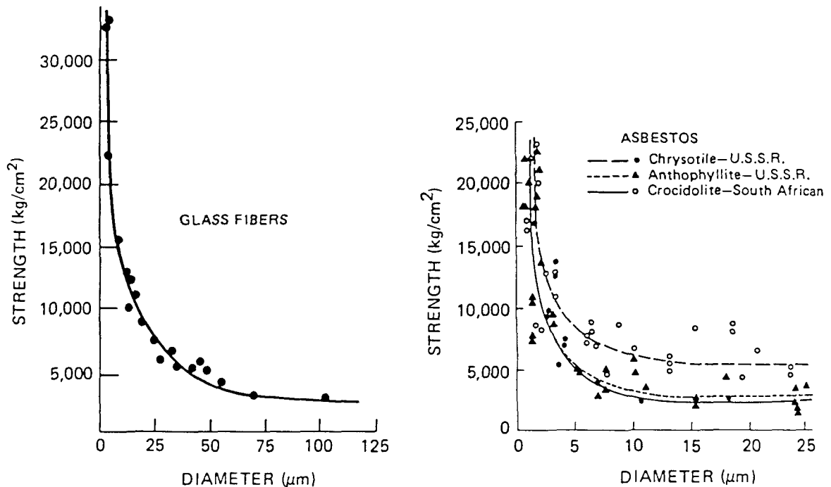
FIGURE 2-4. Illustration of the strength-diameter effect. Data from Griffith, 1921 (glass fibers) and Nadgornyi et al. , 1965 (asbestos).
