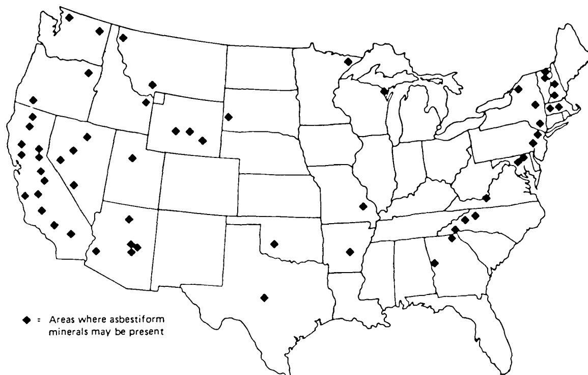
FIGURE 3-4. Areas containing possible asbestiform phases of minerals. From Kuryvial et al. , 1974.
