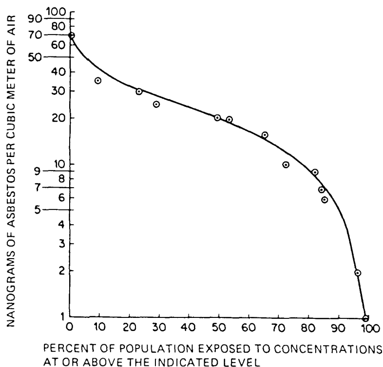
FIGURE 3-1. Distribution of exposures to asbestos in ambient air of urban areas. From Suta and Levine, 1979.
