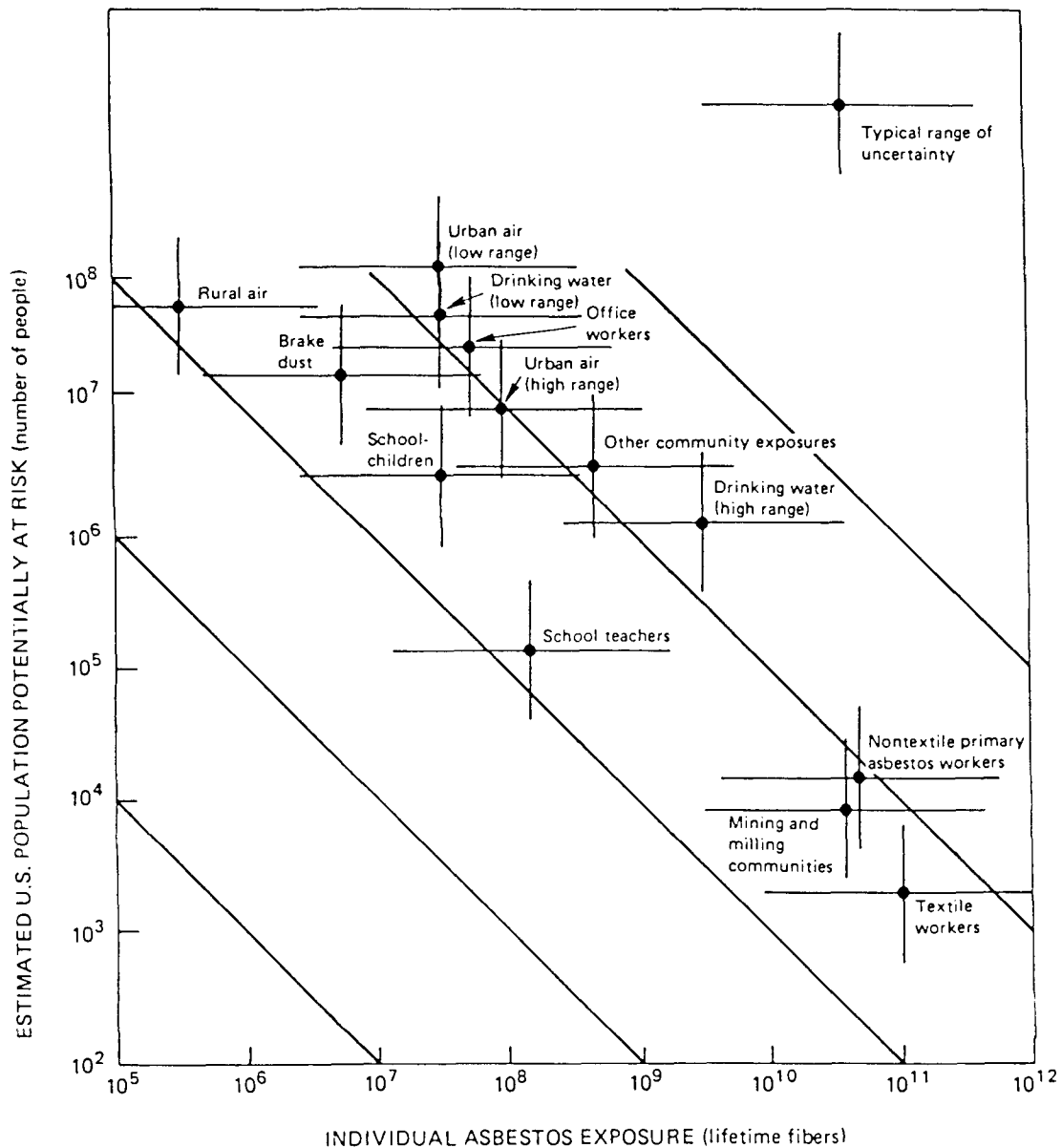
FIGURE 3-3. Estimated lifetime exposures and numbers of people in various groups potentially exposed to asbestos. The points represent approximate estimates, and the lines indicate the ranges of uncertainty. As constructed, the uncertainty is about an order of magnitude for the population estimates and about two orders of magnitude for the exposure estimates. The committee was unable to make explicit estimates of the uncertainty limits, which would vary among the different populations. The points were derived from measurements or models for the groups represented; many of the points (e.g., the schoolchildren point) can be traced back to data provided in the section in this chapter entitled Quantitative Exposure Estimates.
