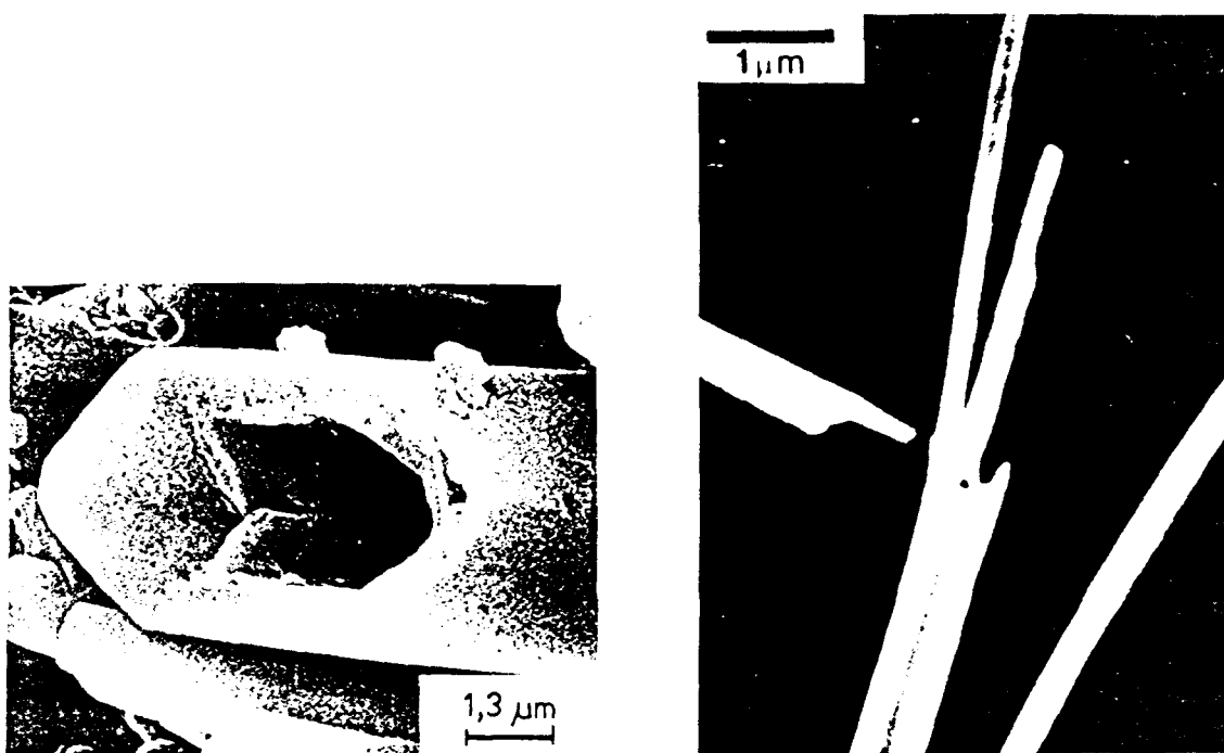
FIGURE 2-5. The dissolution pattern of a glass fiber (from Wojnárovits-Hrapka, 1977) and amosite fibers (from Walker, 1981).
