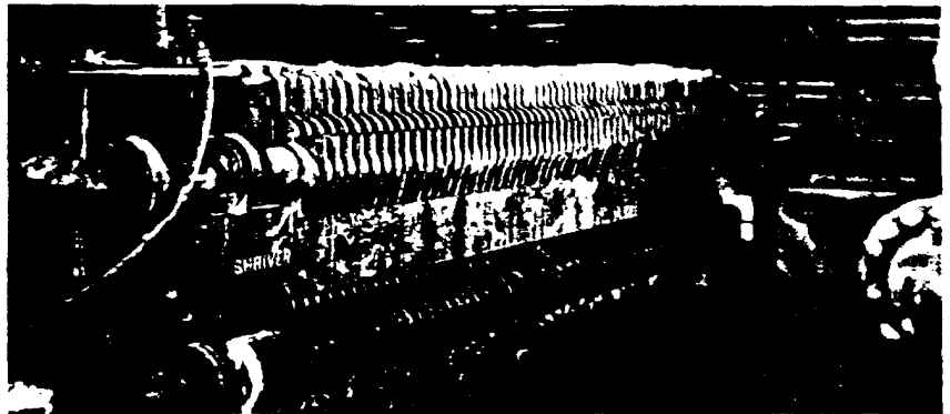
Lead coated filter plates and frames in use
