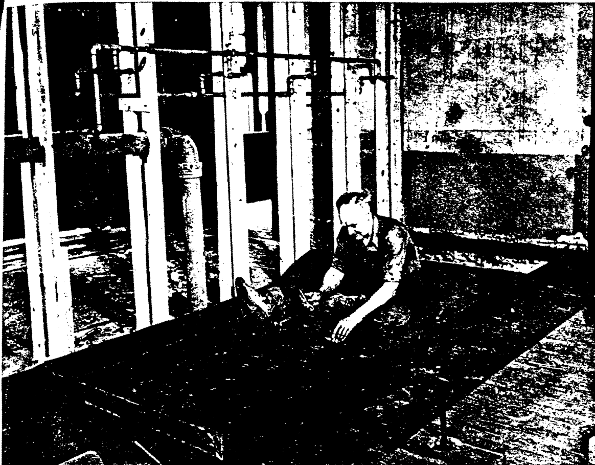
Installing lead pan for shower battery in dormitory for Navy personnel at Georgia School of Technology. Note builders felt under pan to be turned up around edges. Inside of pan will be coated with asphalt before setting tile
