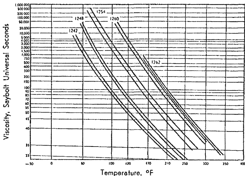
Fig. 4—VISCOSITY RANGES OF SOME AROCLORS
