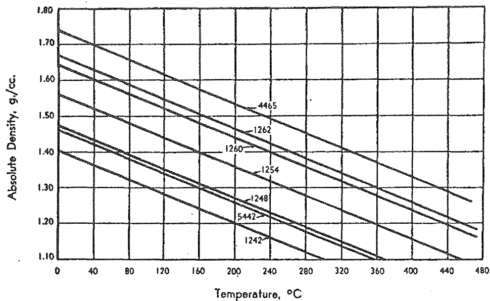
Fig. 2. DENSITIES OF AROCLORS AT VARIOUS TEMPERATURES
