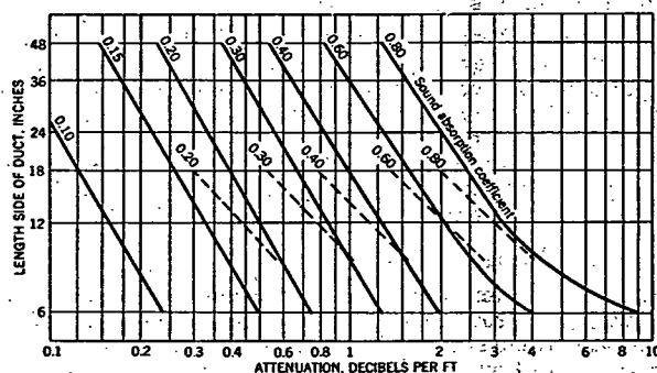
FIG. 3. SOUND ATTENUATION FOR VARIOUS ABSORBING DUCT LINERS
