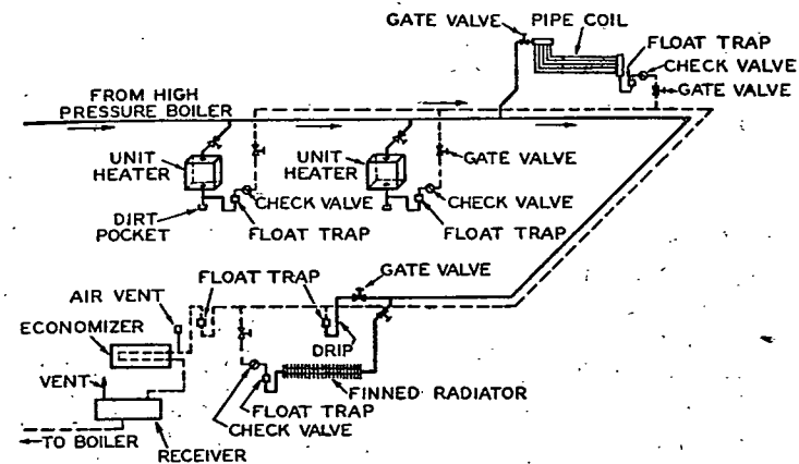
FIG. 8. TYPICAL HIGH PRESSURE HEATING SYSTEM
