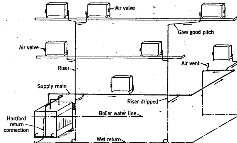
FIG. 6. TYPICAL UP-FEED GRAVITY ONE-PIPE AIR-VENT SYSTEM
