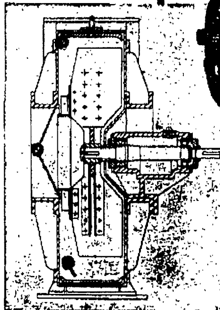
At left - Section through mill exhaustor showing new shrouded fan wheel with "schlizer" blades.
