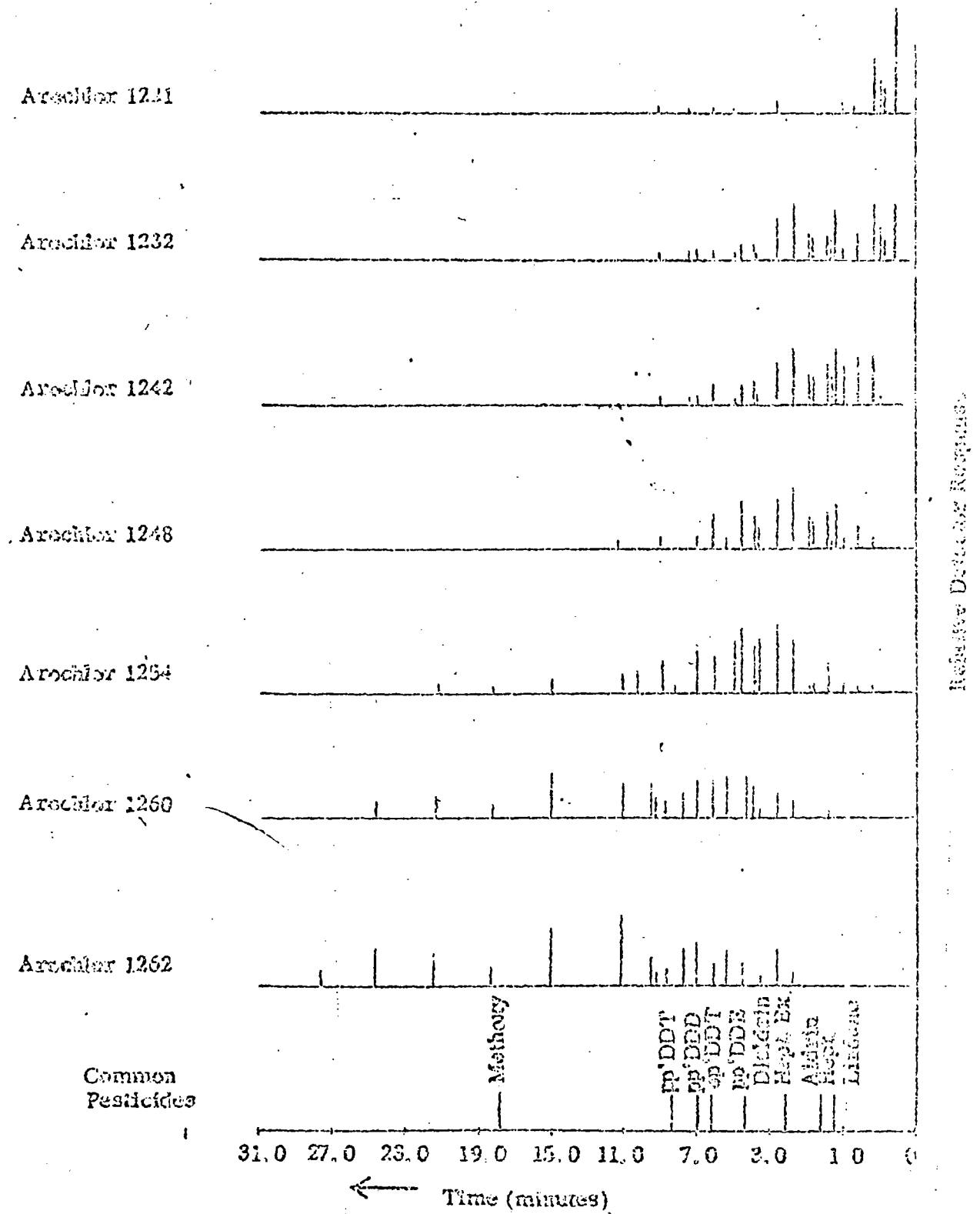
Figure 3, Simulated Chromatograms of the Aroclors
