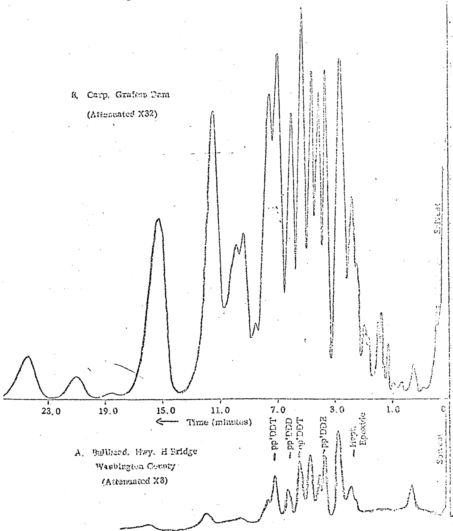
Figure 6. Fish Chromatograms from Lake Erie
