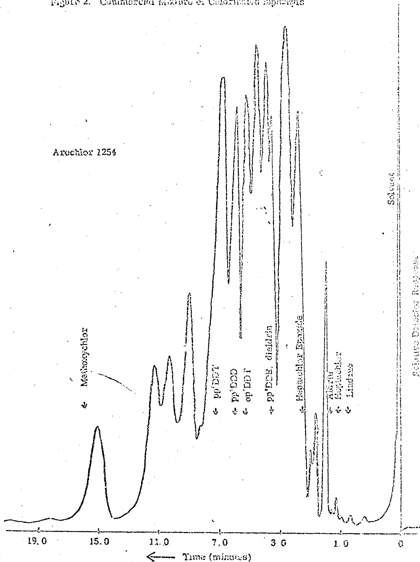
Figure 2. Commercial Mixture of Chlorinated Biphenyls
