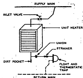
FIG. 53. TYPICAL UNIT HEATER CONNECTIONS FOR TWO-PIPE SYSTEM
