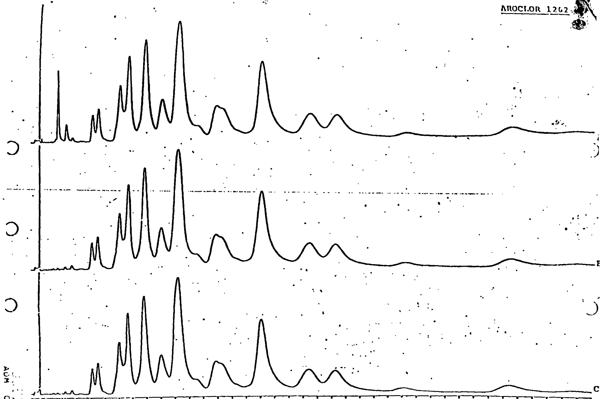
FIGURE 6. Electron capture gas chromatographic trace of (A) Aroclor 1262 and treated with 1:1 mixture of nitric and sulfuric acids and extracted into hexane, (B) Aroclor 1262 treated with distilled water and extracted into hexane, and (C) untreated Aroclor 1262 standard in hexane.
