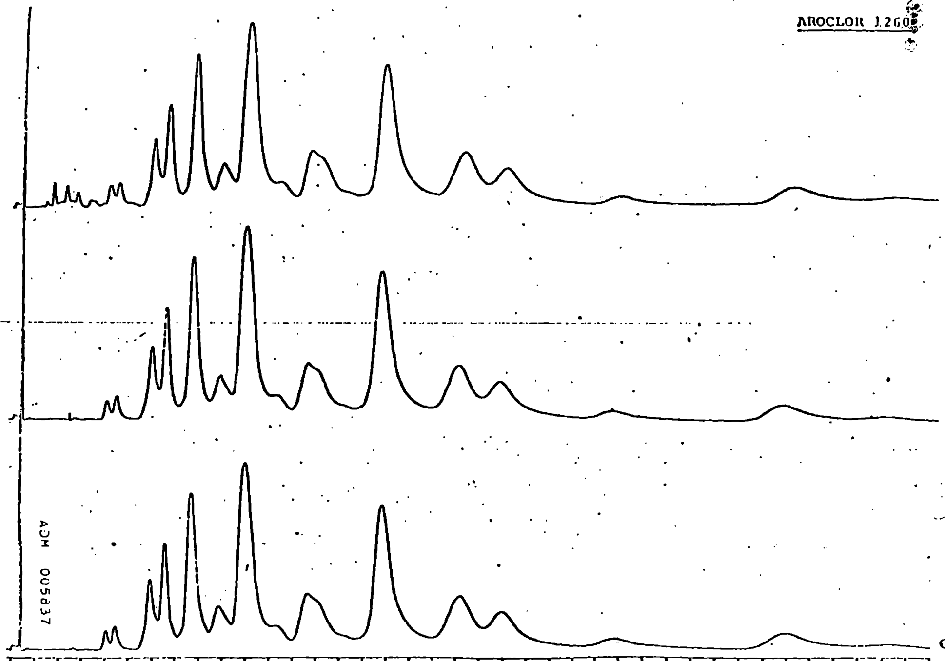
FIGURE 5. Electron capture gas chromatographic trace of (A) Aroclor 1260 and treated with 1:1 mixture of nitric and sulfuric acids and extracted into hexane, (B) Aroclor 1260 treated with distilled water and extracted into hexane, and (C) untreated Aroclor 1260 standard in hexane.
