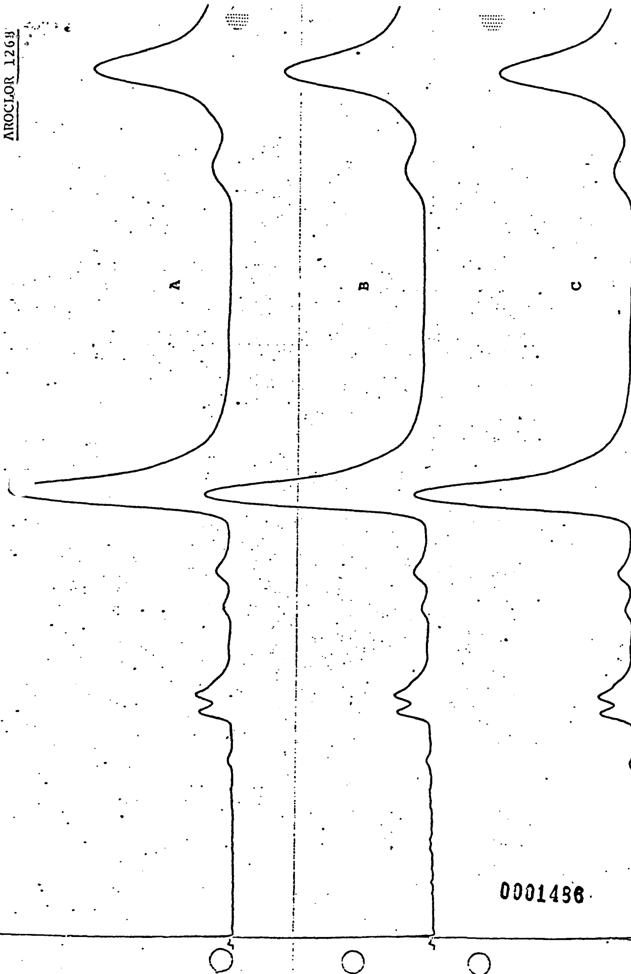
FIGURE 7. Electron capture gas chromatographic trace of (A) Aroclor 1268 and treated with 1:1 mixture of nitric and sulfuric acids and extracted into hexane, (B) Aroclor 1268 treated with distilled water and extracted into hexane, and (C) untreated Aroclor 1268 standard in hexane.
