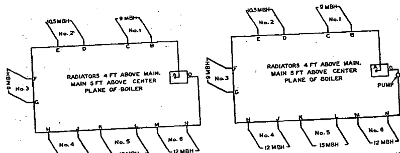
FIG. 10. ONE-PIPE GRAVITY CIRCULATION SYSTEM (EXAMPLE 3)
