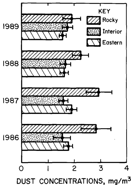
Figure 14.—Average dust compliance concentrations of provinces surveyed.
